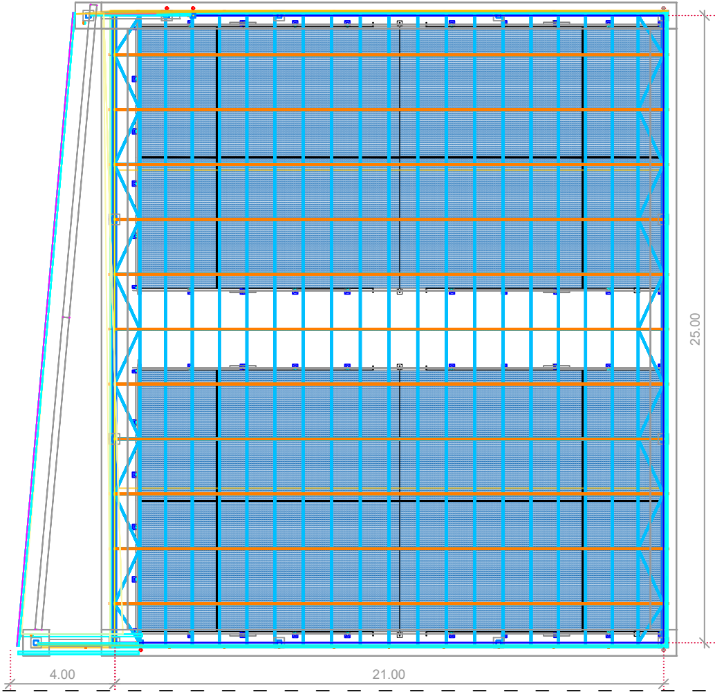
THONGSBRIDGE_FLOOR PLAN_E: 1/200
