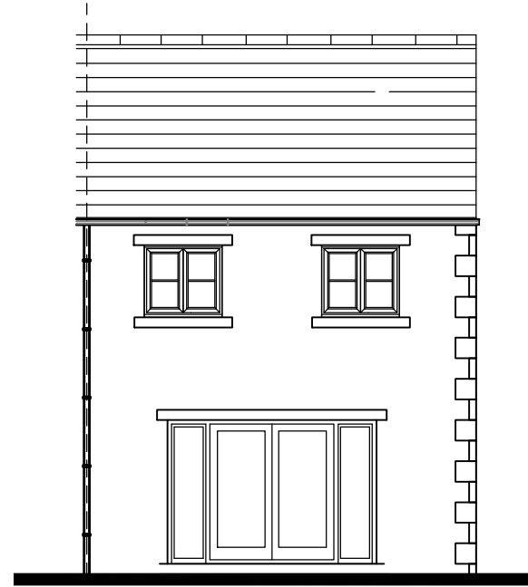
Rear elevation 1:100
