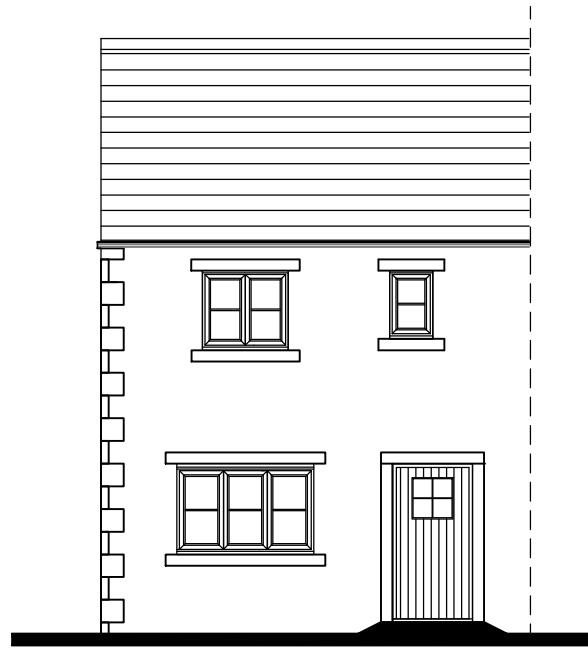
Front elevation 1:100
