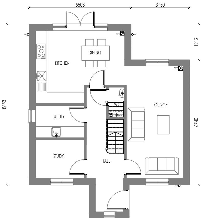
Ground floor 1:100
