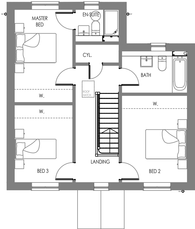
First floor 1:100
