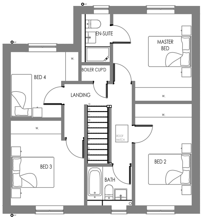
First floor 1:100
