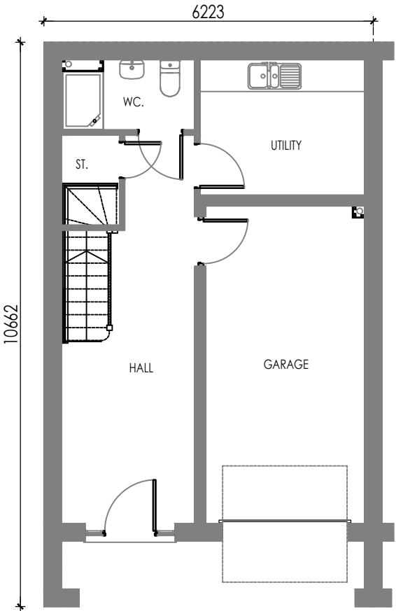
Lower ground floor 1:100
