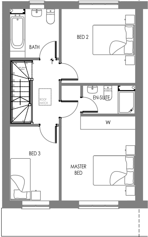
First floor 1:100
