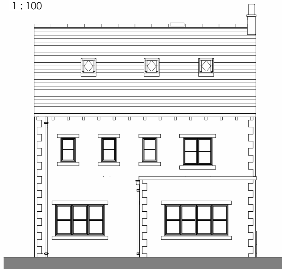
Rear Elevation
