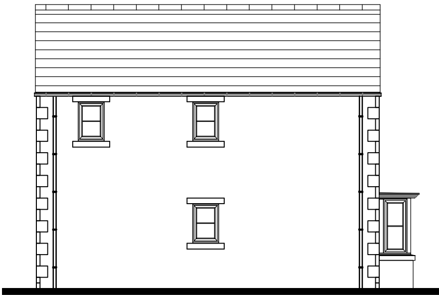
Rear elevation 1:100
