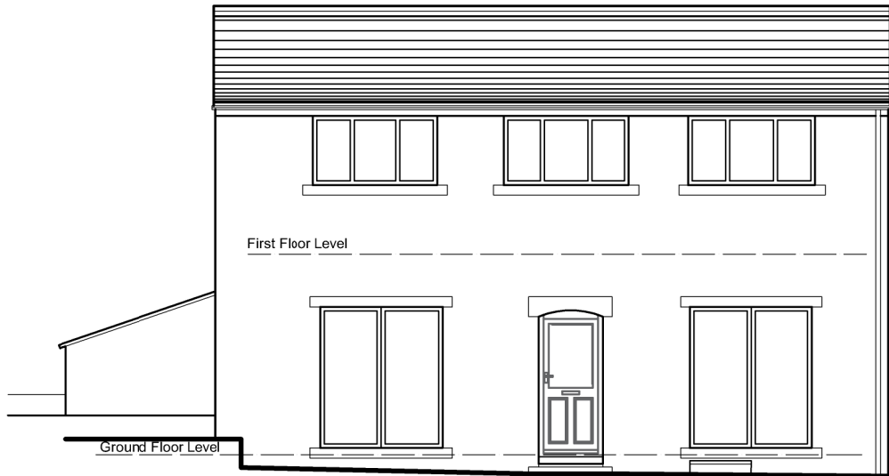
South East Elevation (Front)
