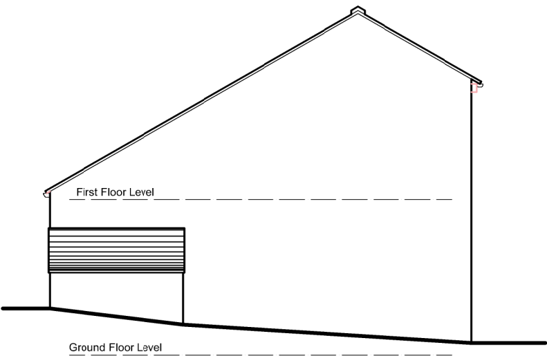
South West Elevation (Side)
