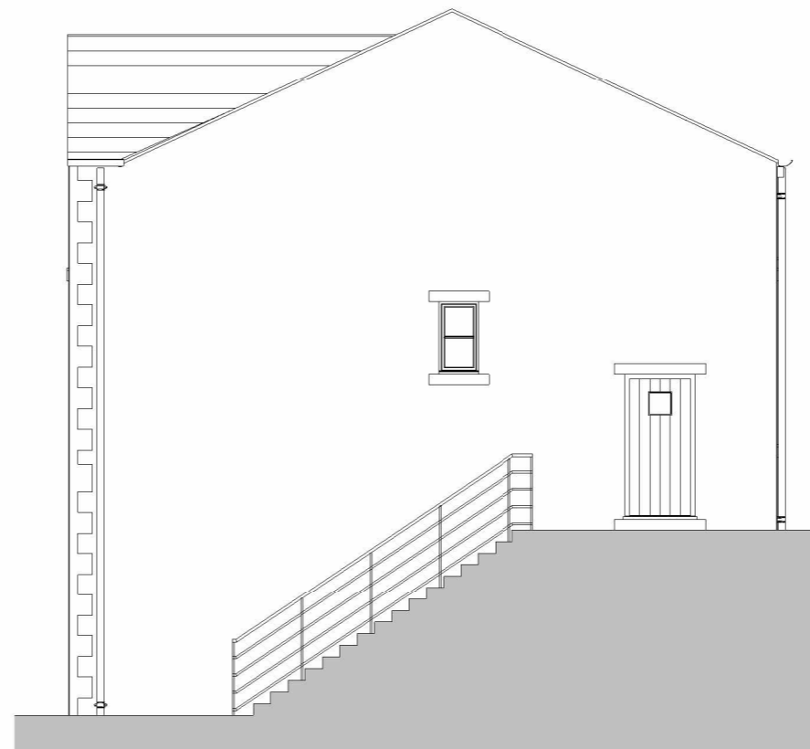
Side elevation 1 : 100
