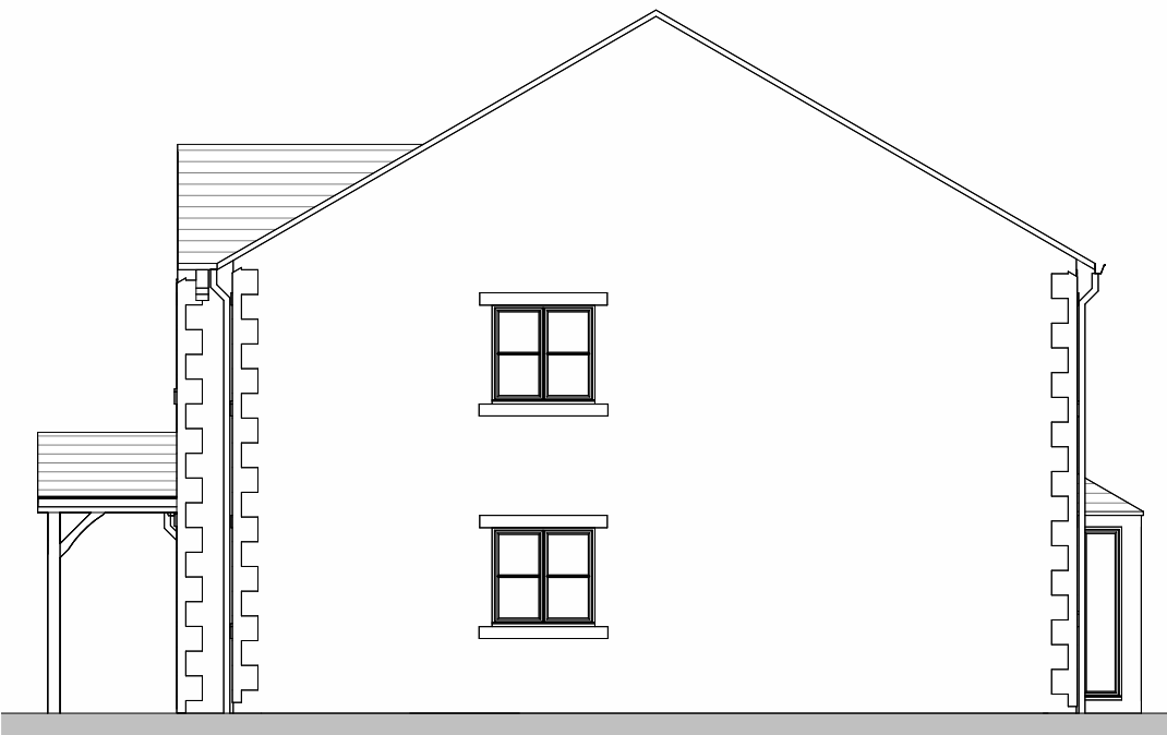
Side Elevation 1 : 100
