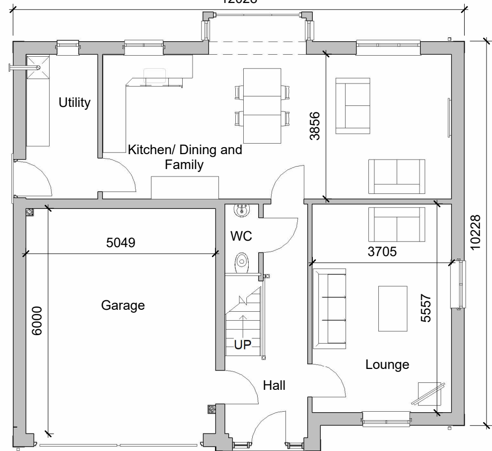
Ground floor 1 : 100
