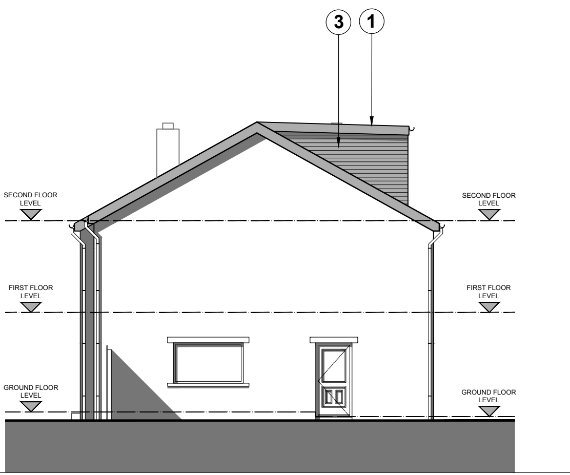
PROPOSED WEST ELEVATION SCALE - 1:50
