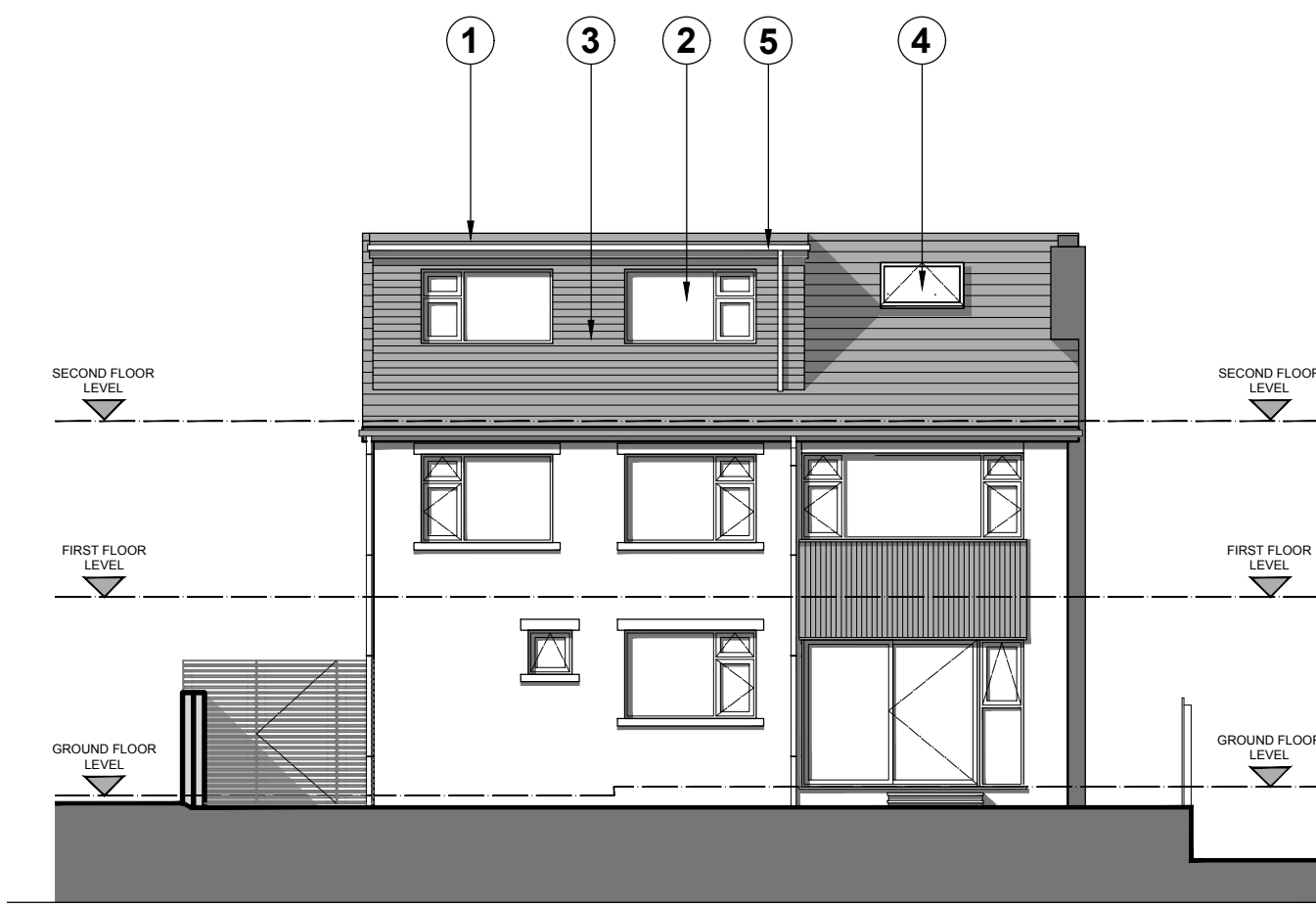
PROPOSED SOUTH ELEVATION SCALE - 1:50
