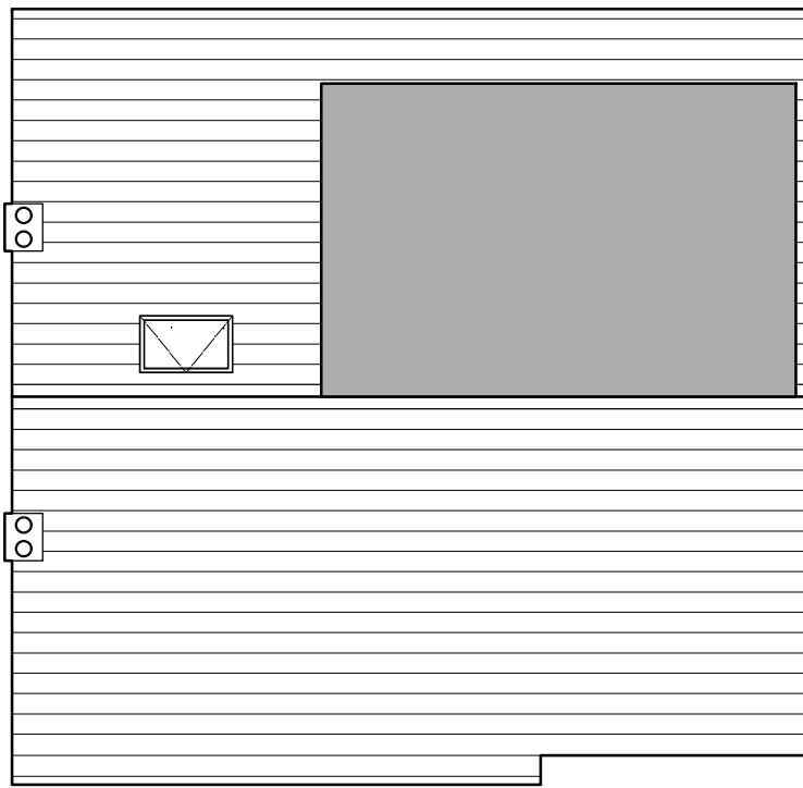
PROPOSED ROOF FLOOR PLAN SCALE - 1:100
