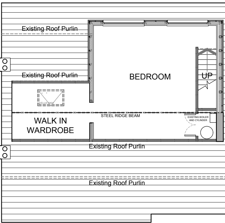
PROPOSED LOFT FLOOR PLAN SCALE - 1:100
