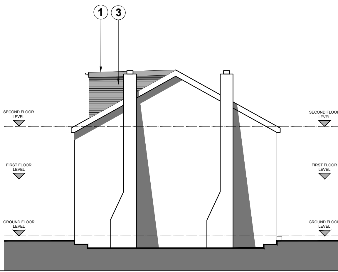
PROPOSED EAST ELEVATION SCALE - 1:50
