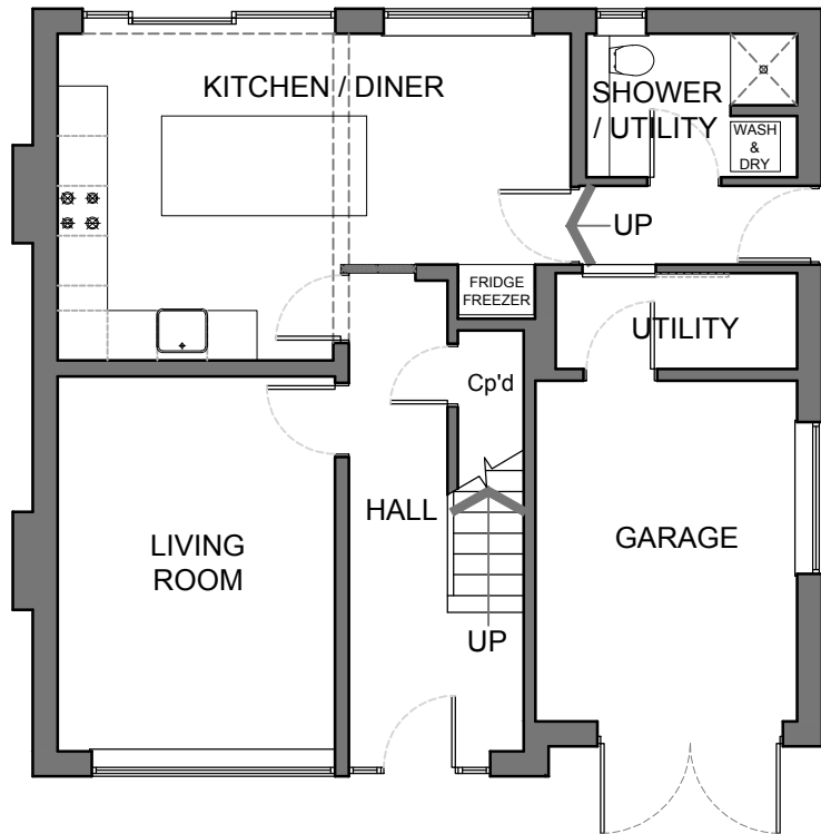
PROPOSED GROUND FLOOR PLAN SCALE - 1:100
