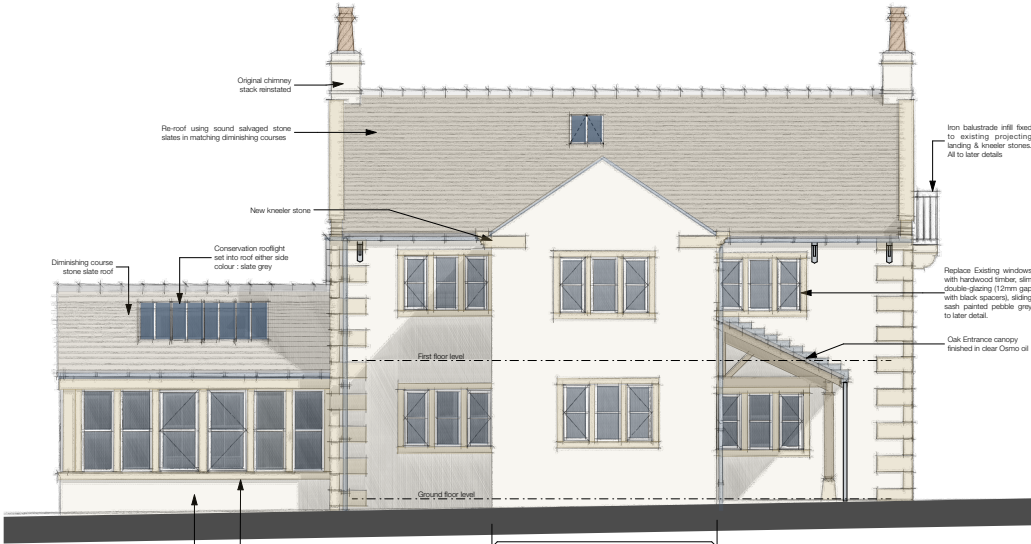
Proposed West Elevation - 1:50
