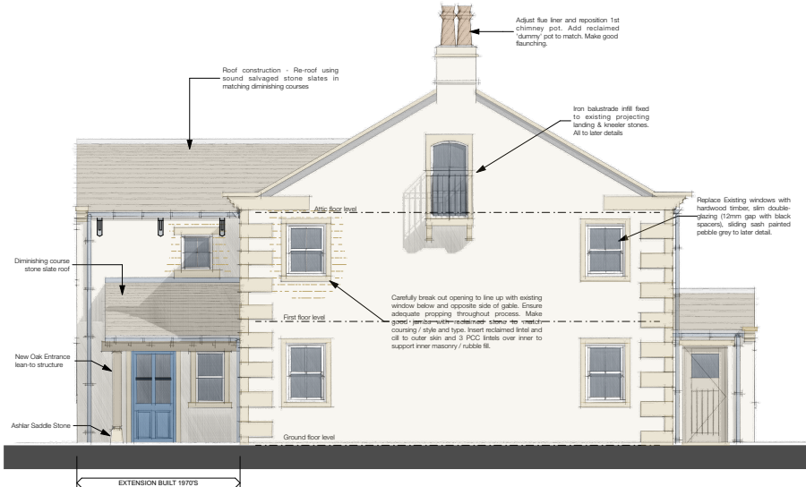
Proposed South Elevation - 1:50
