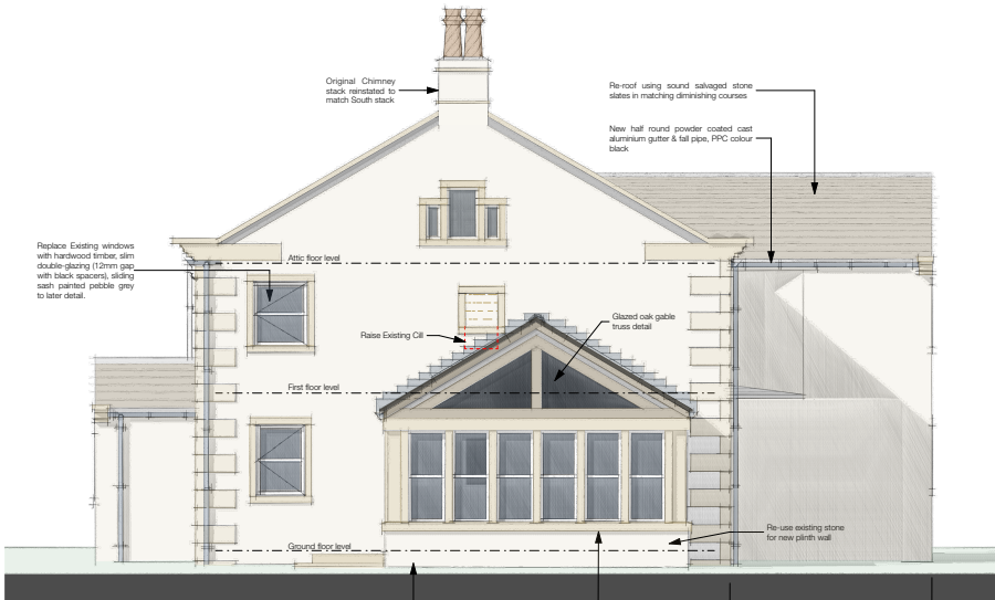
Proposed North Elevation - 1:50
