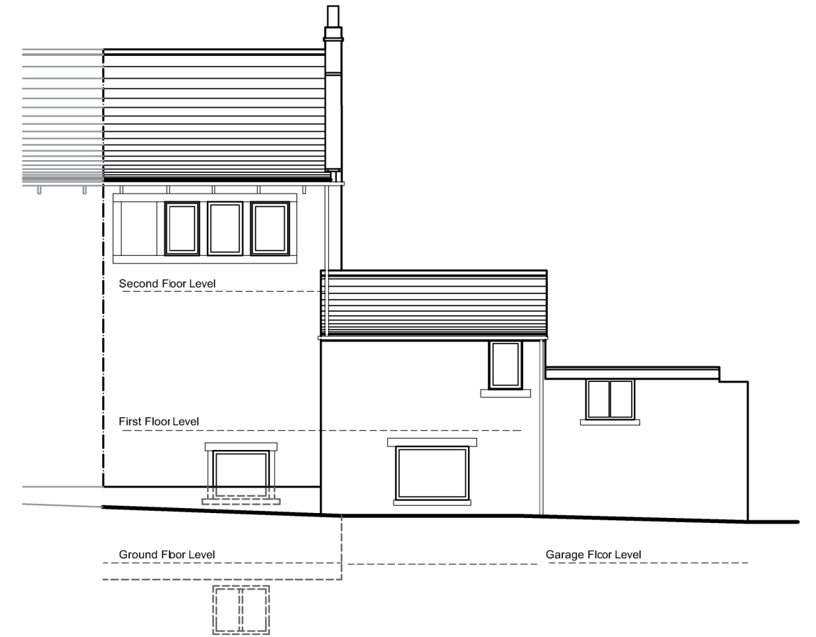
North Elevation
