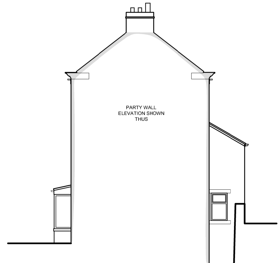
East Elevation
