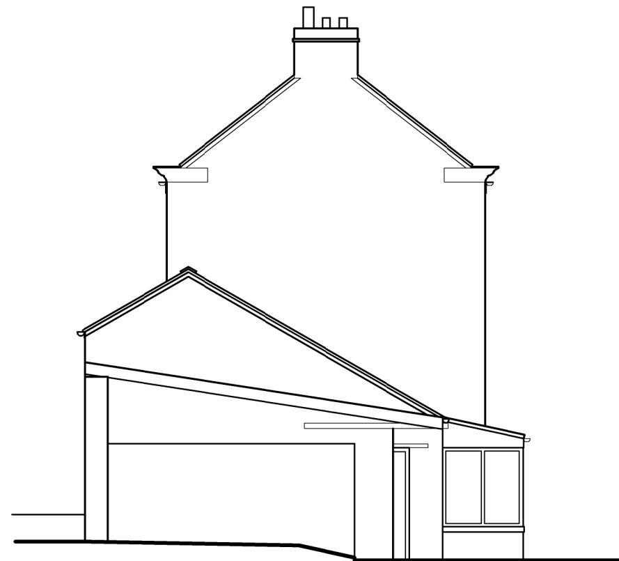
West Elevation
