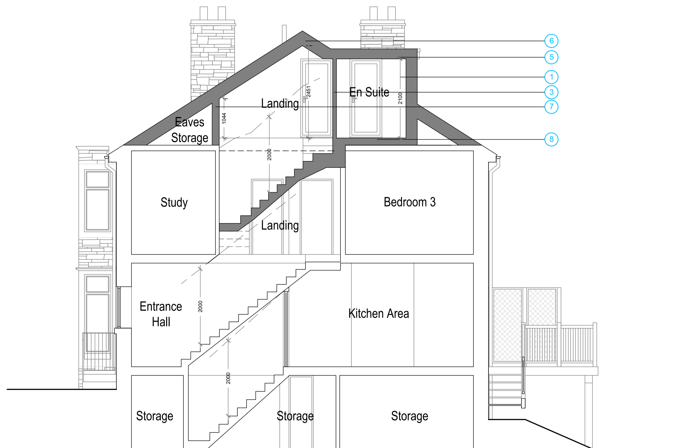
Proposed Section A-A Scale 1:50
