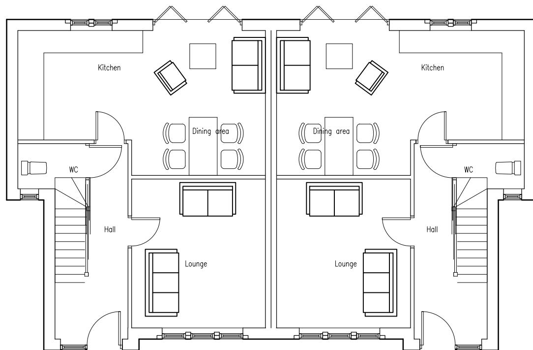
Ground Floor Layout
