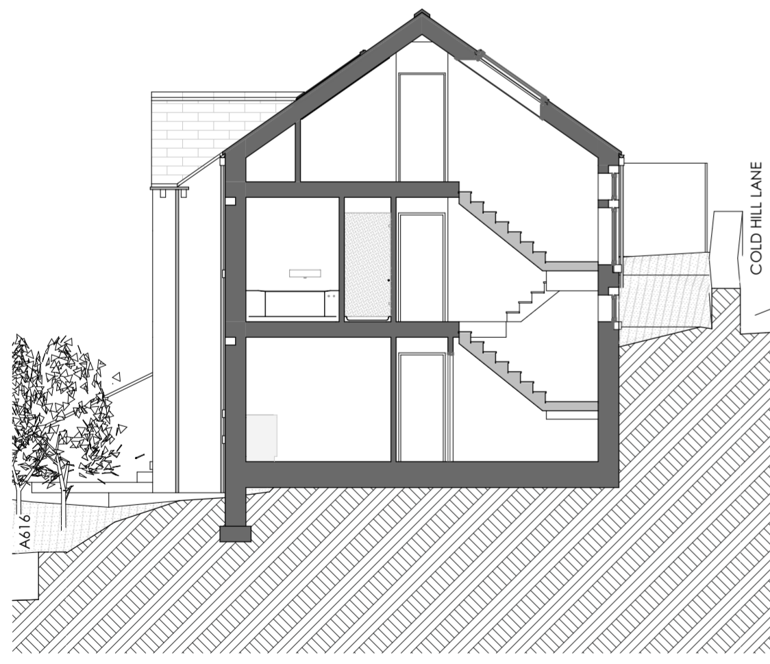
01 Building Section 1:100
