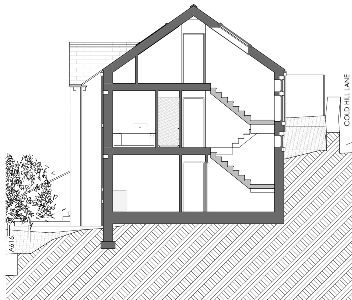
01 Building Section 1:100
