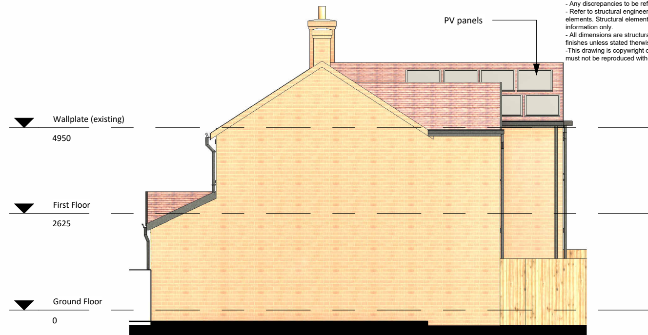
3 11 EAST Proposed 1 : 100
