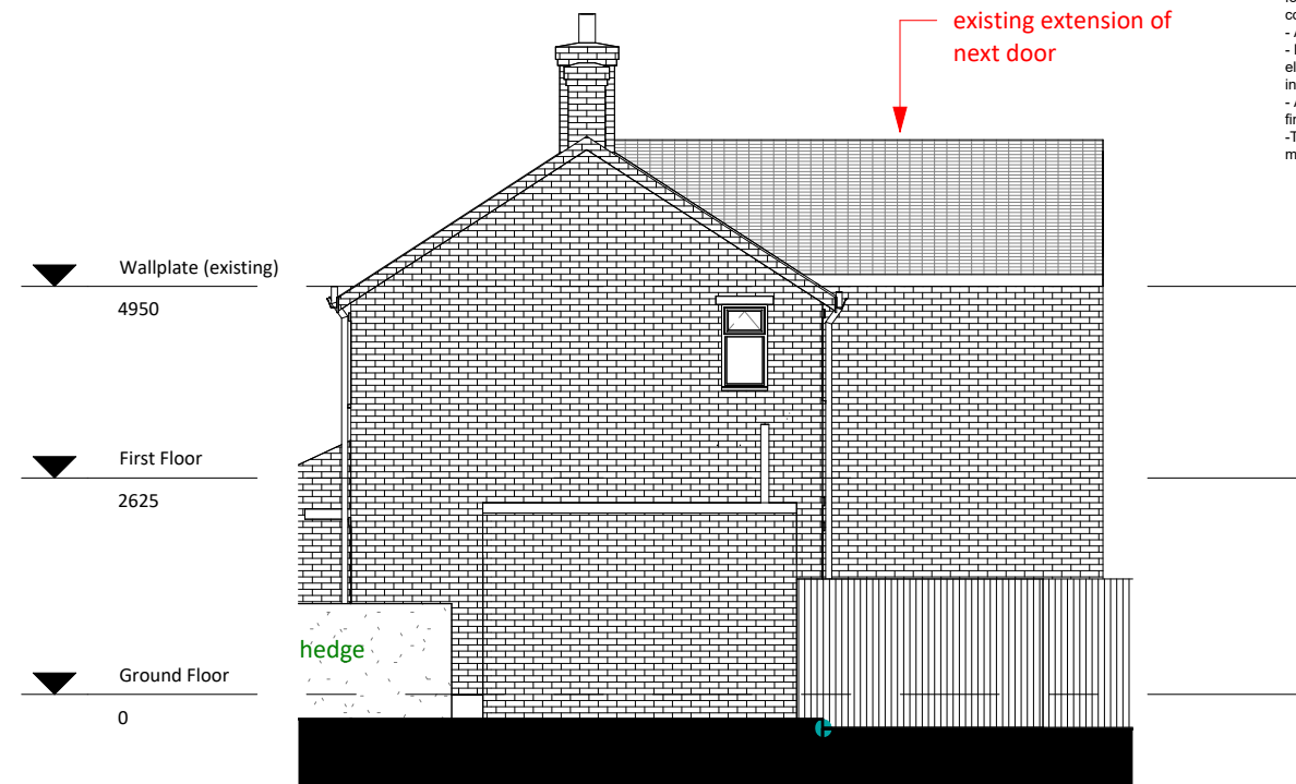
10 EAST Existing 1 : 100
