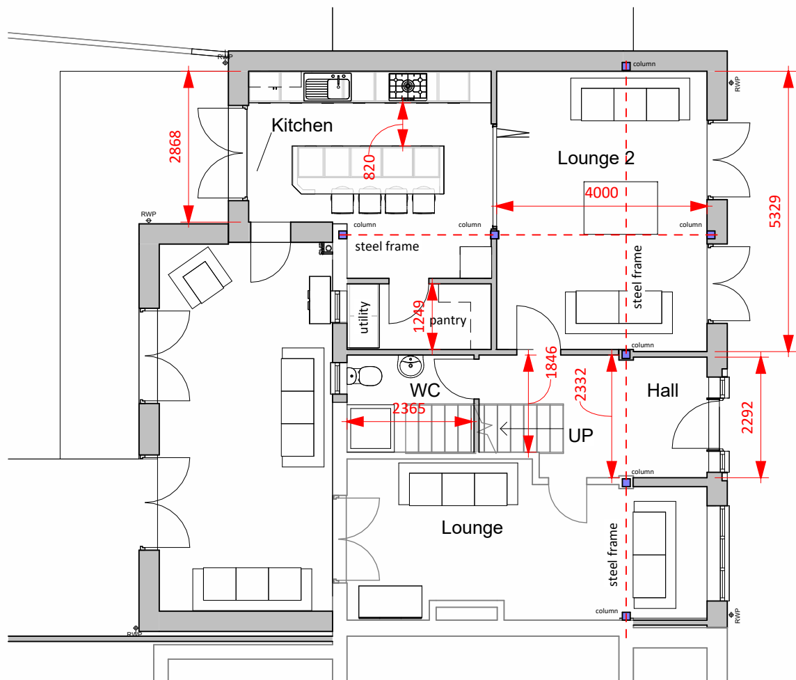
1 02b GF Proposed 1 : 100
