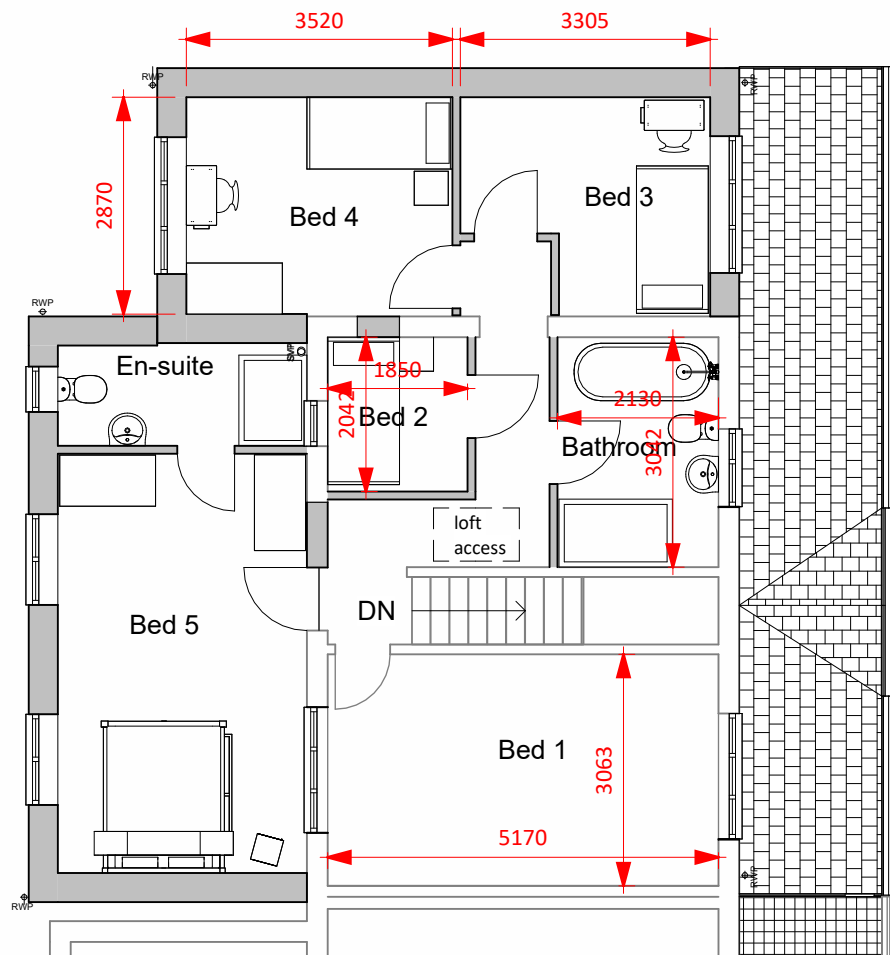
03b FF Proposed 1 : 100
