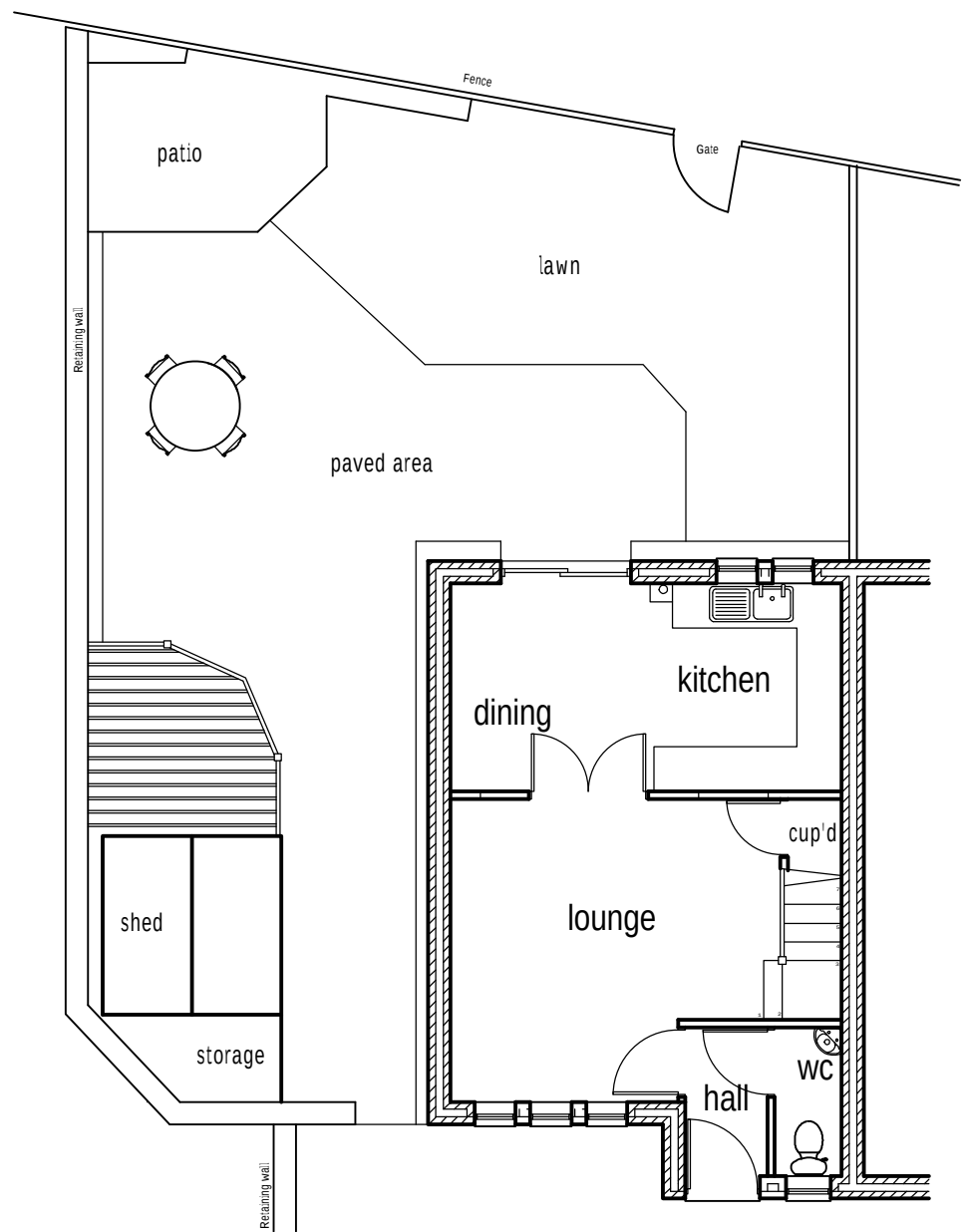
Existing Ground Floor Layout (1:100)
