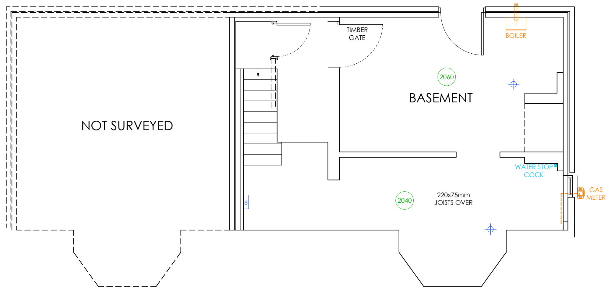
BASEMENT PLAN
