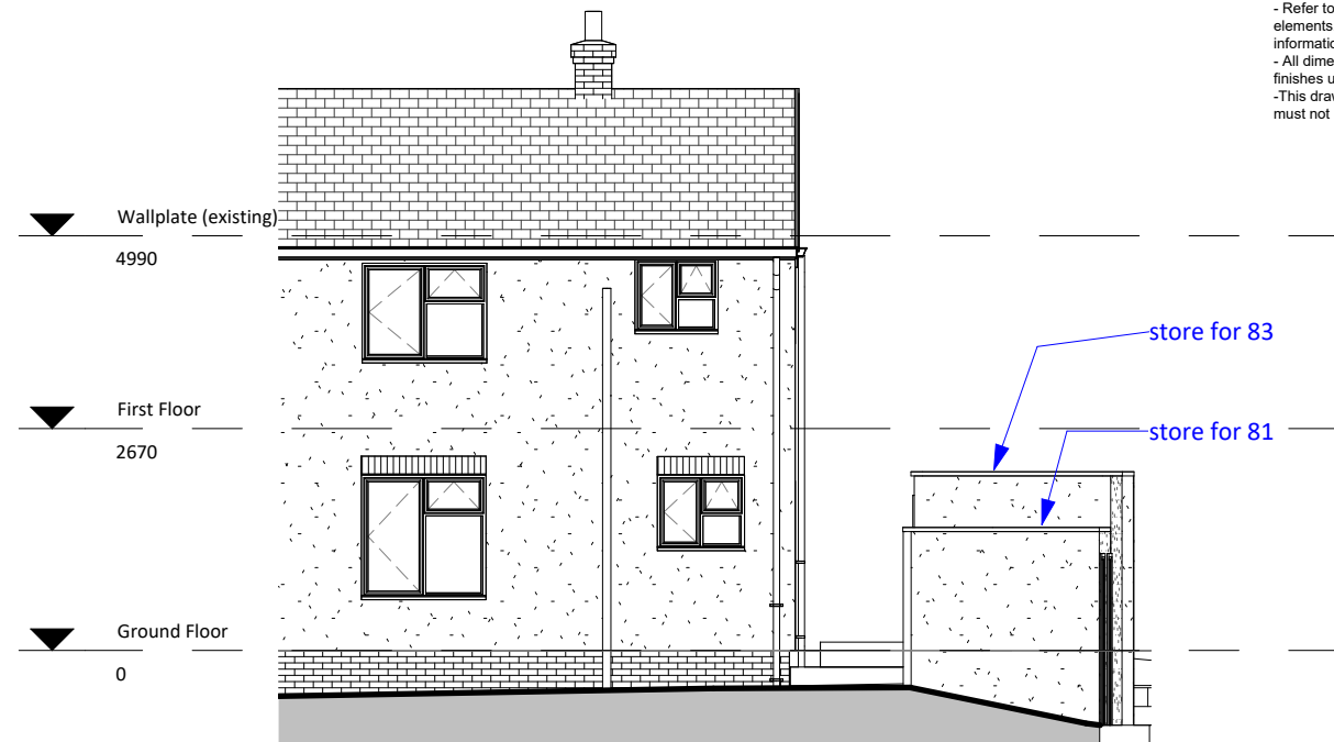
2 10 South West Existing 1 : 100
