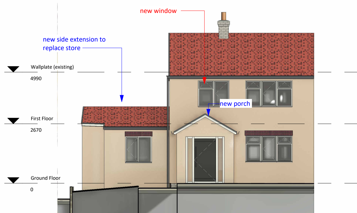
1 11 North East Proposed 1 : 100
