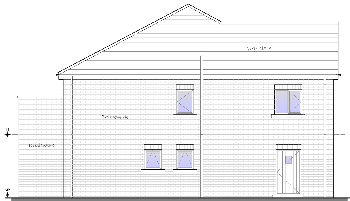
PROPOSED NORTH-WEST (SIDE) ELEVATION SCALE - 1:100
