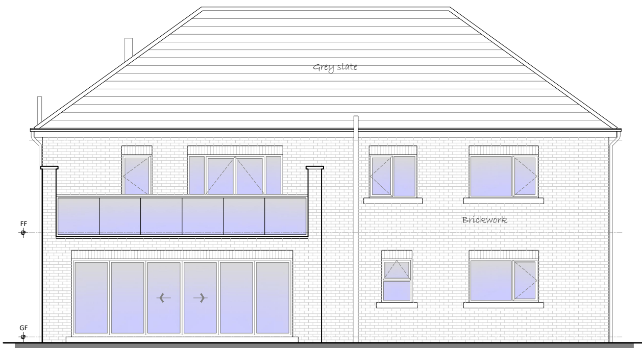
PROPOSED NORTH-EAST (REAR) ELEVATION SCALE - 1:100
