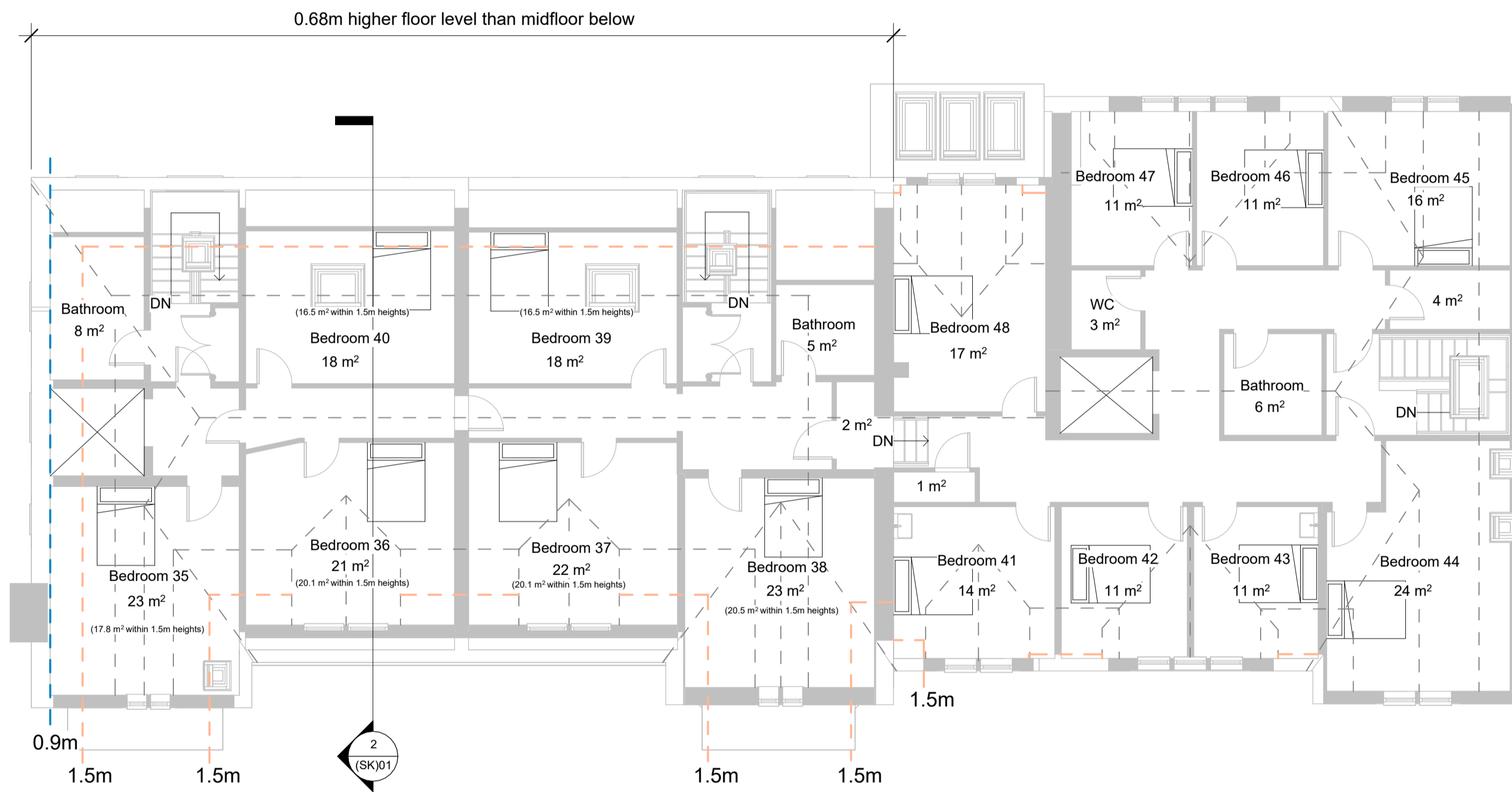
1 Second Floor Proposed Heights 1:100
