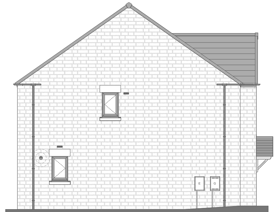
Left Elevation
