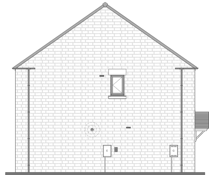
Left Elevation
