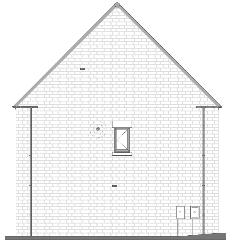
Left Elevation
