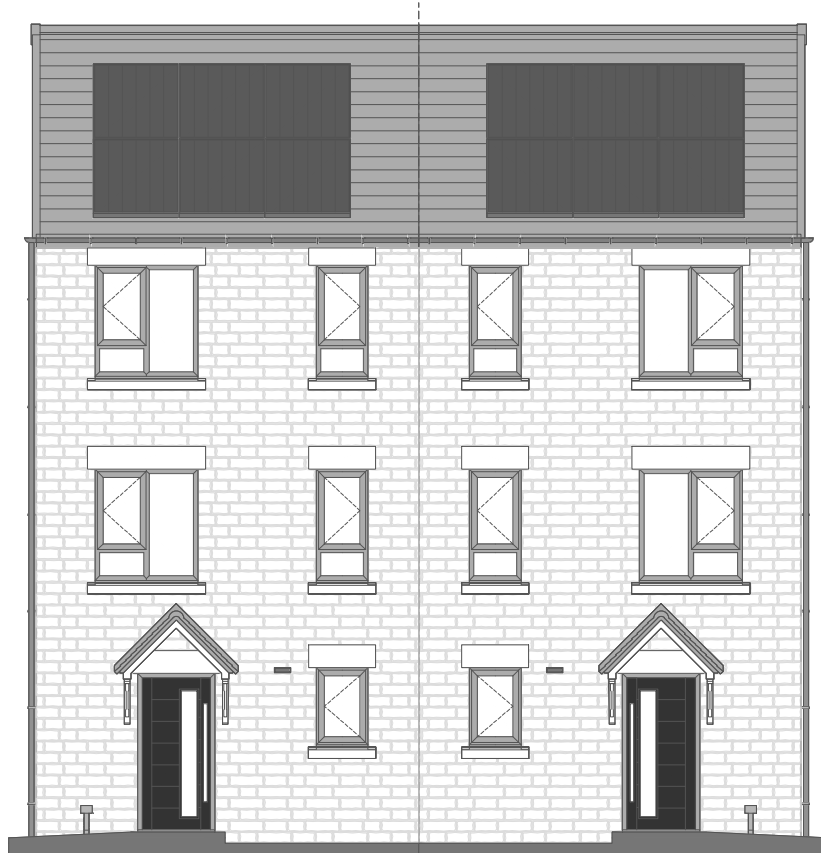
Front Elevation
