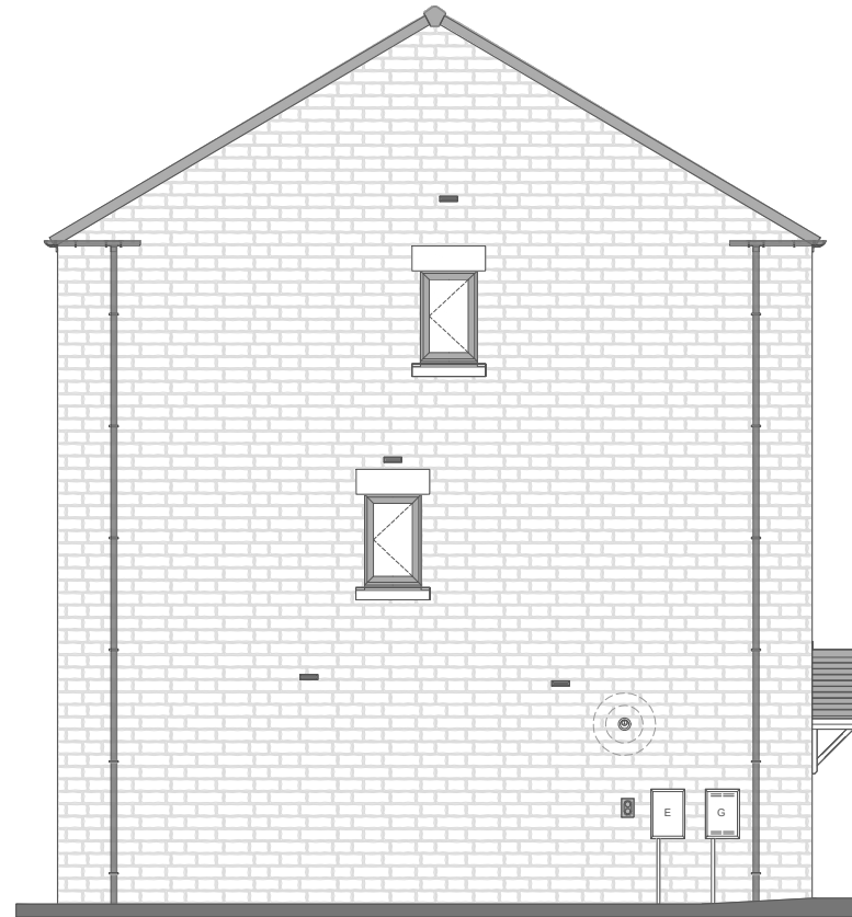
Left Elevation
