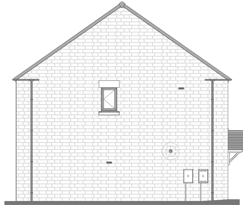
Left Elevation
