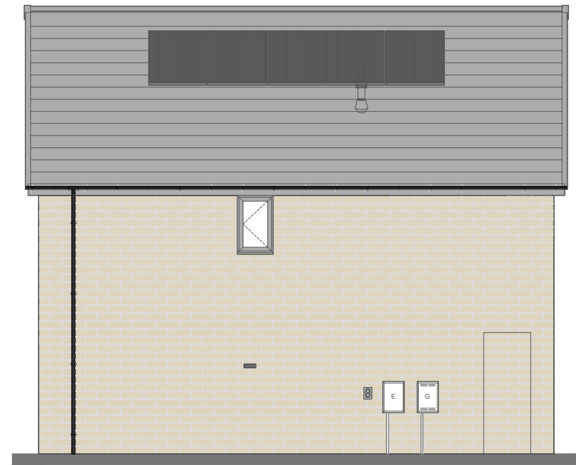
Left Elevation
