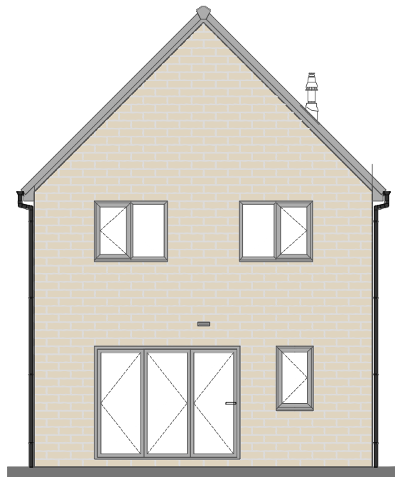
Rear Elevation
