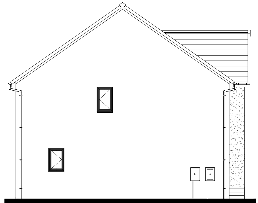
Left Elevation
