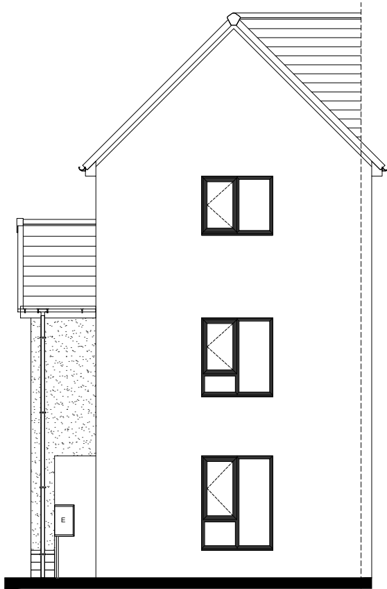
Front Elevation
