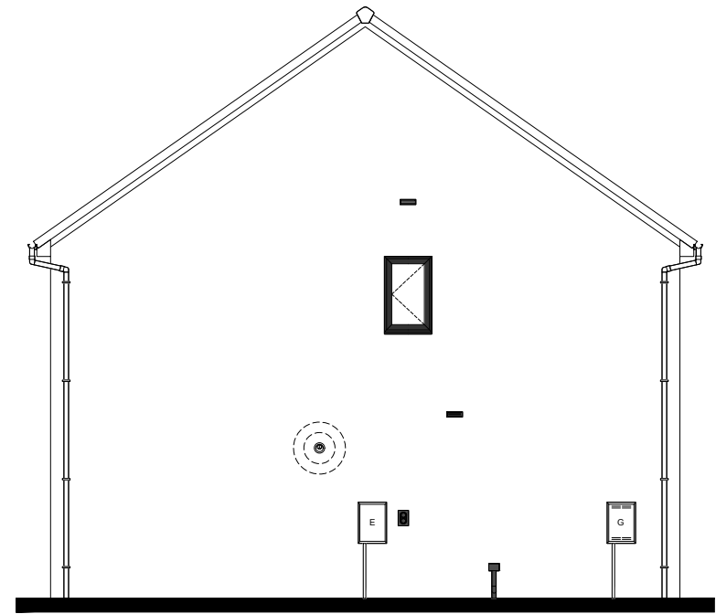
Left Elevation
