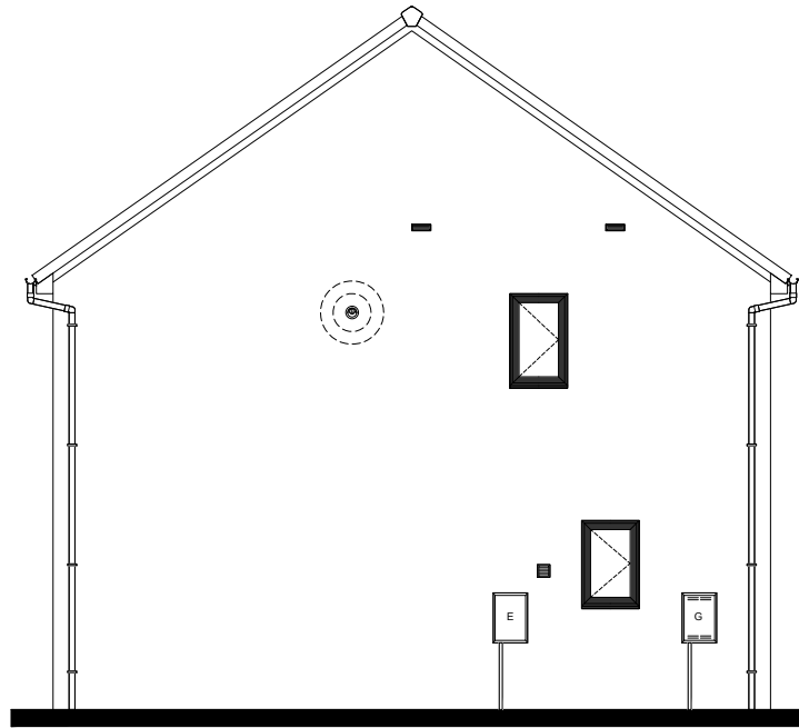
Left Elevation
