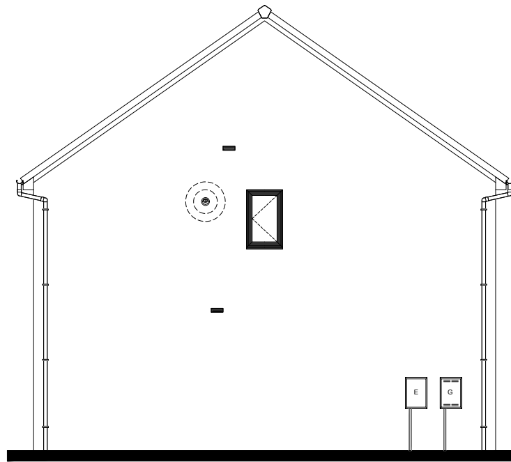
Left Elevation
