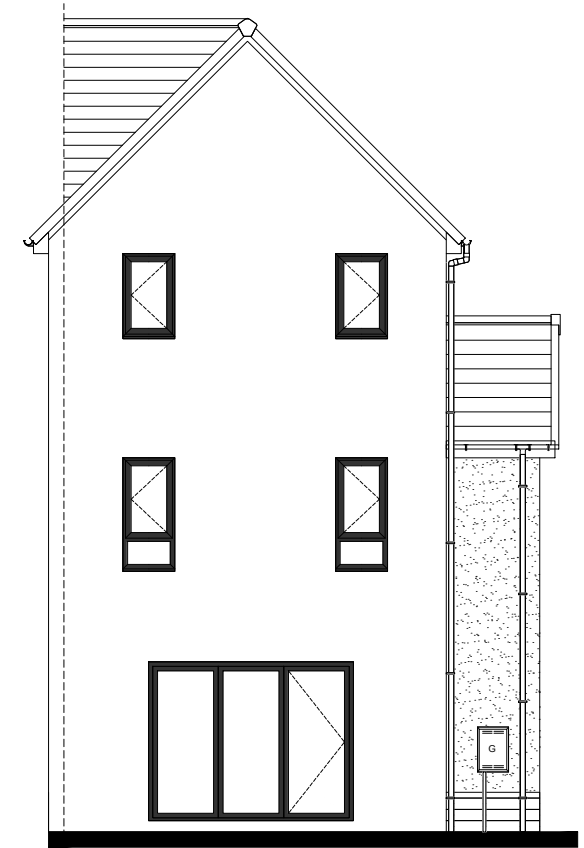
Rear Elevation
