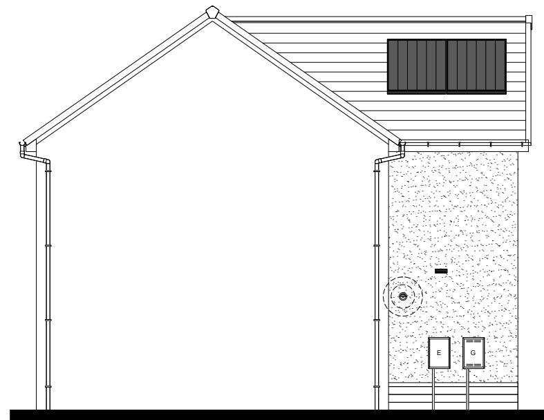
Left Elevation
