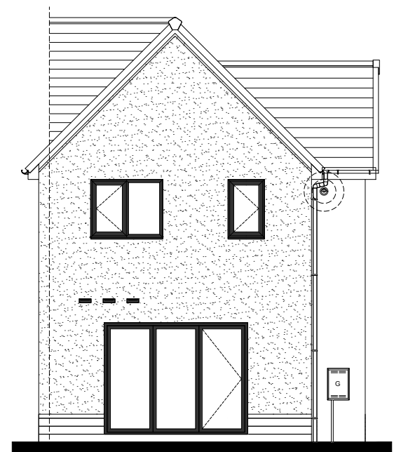
Rear Elevation
