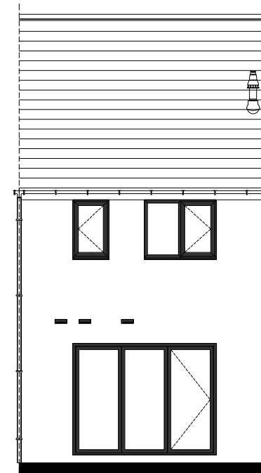
Rear Elevation
