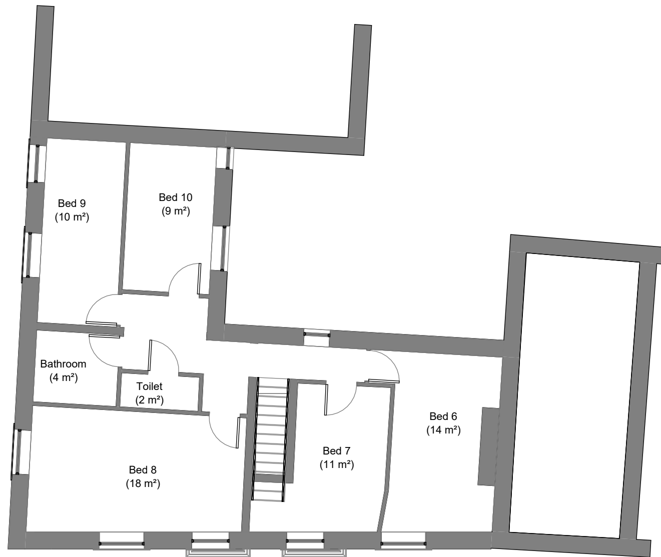
1 First Floor Plan 1 : 100
