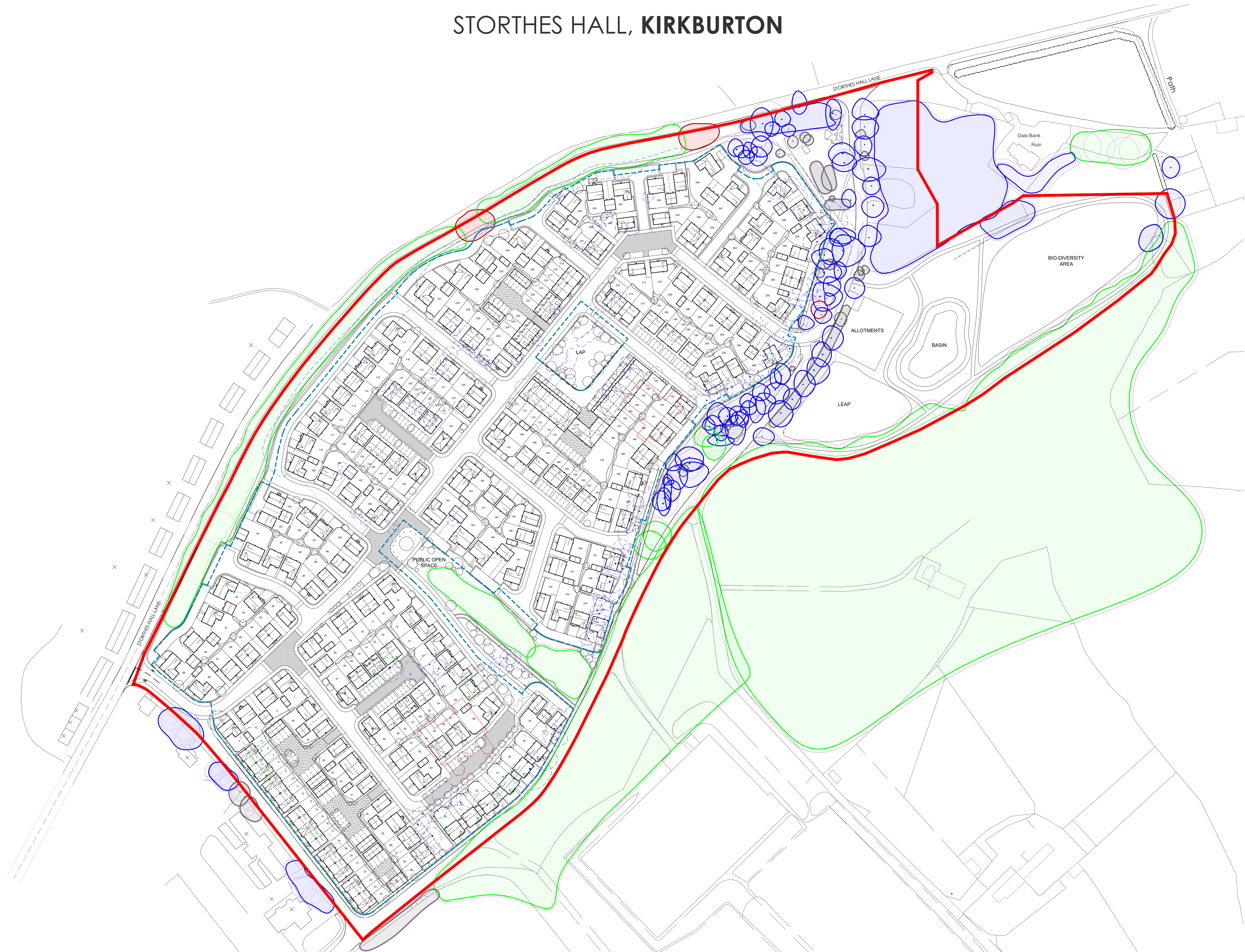
Site Layout Plan with Tree Root Protection Areas - Scale 1:1000
