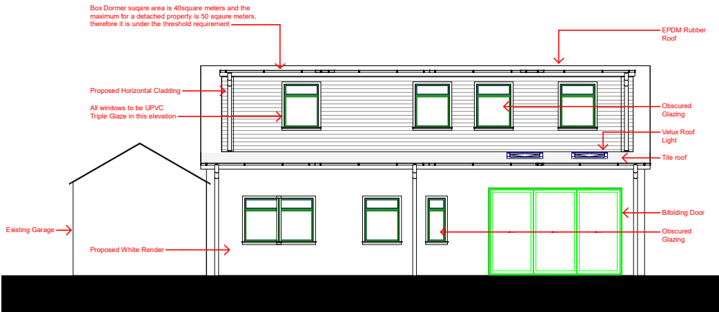
Proposed South Elevation (Rear)
