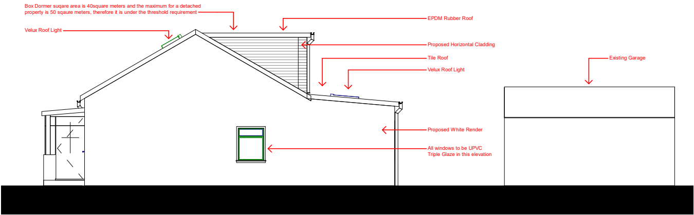
Proposed East Elevation (Right Side Elevation)
