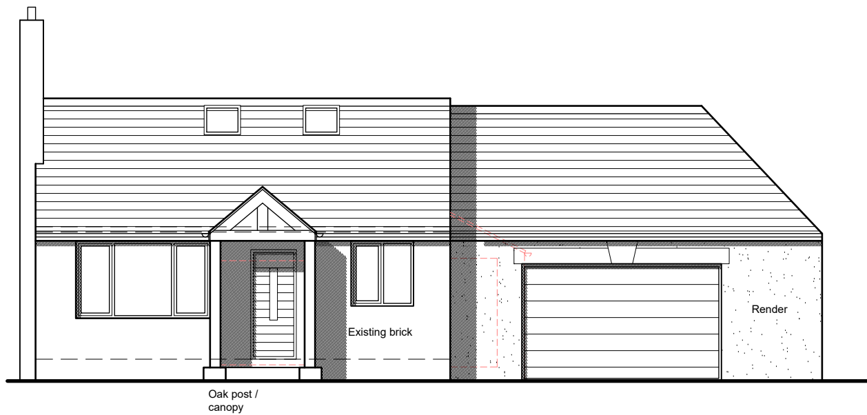
South Elevation
