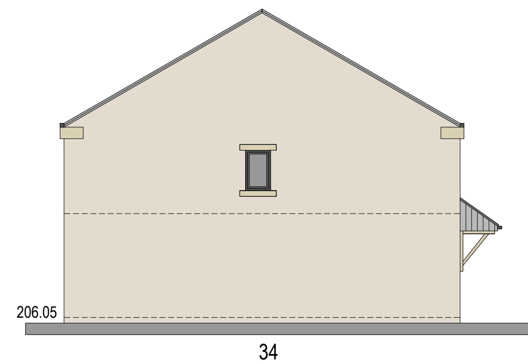
WEST ELEVATION
