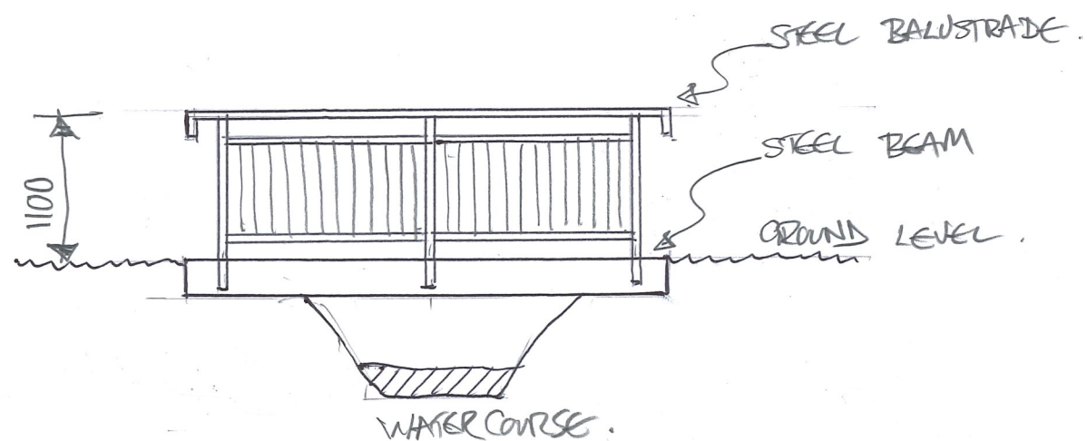
SECTIONAL ELEVATION (1:50)
