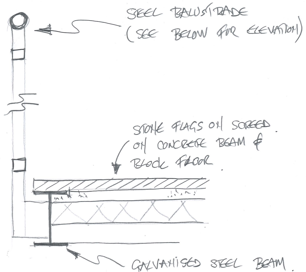
CROSS SECTION THRO' BRIDGE (1:10)
