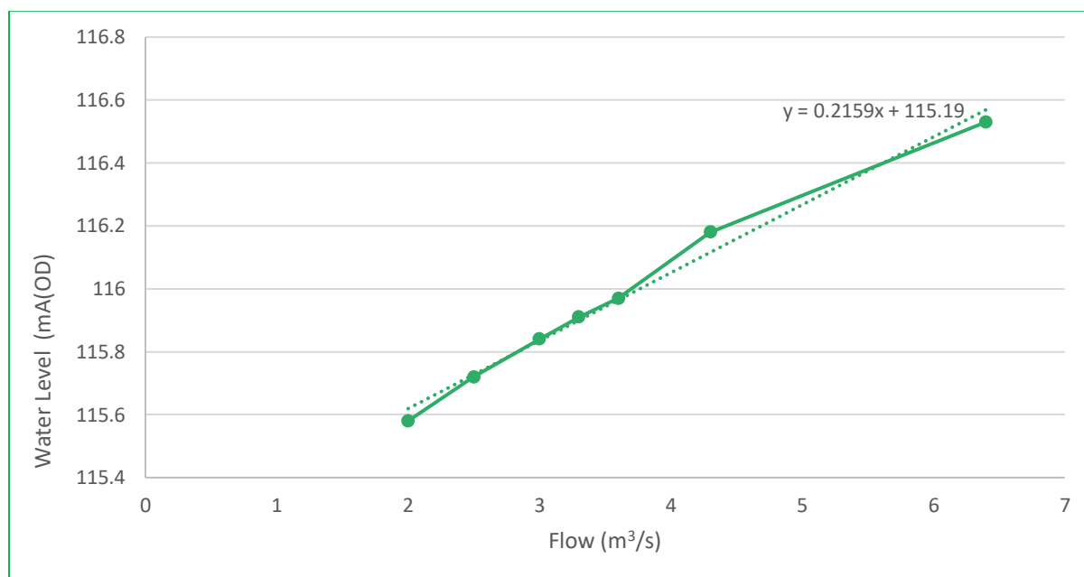
Figure 4 - Rating Curve
