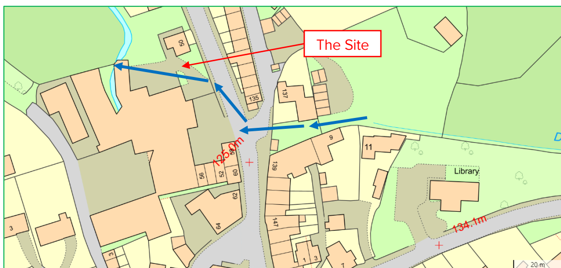
Figure 6 - Overland Flow Path
