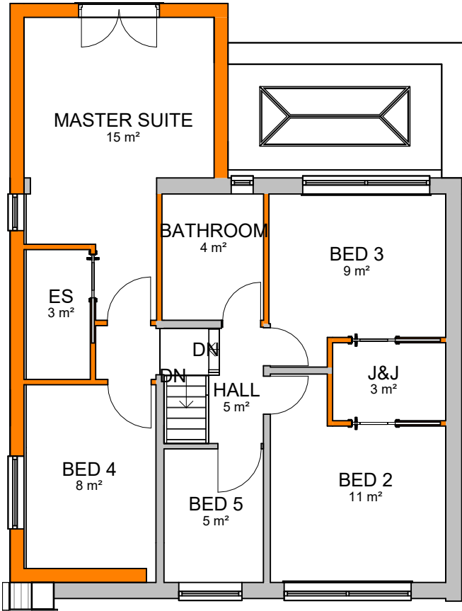
Proposed First Floor 1 : 100
