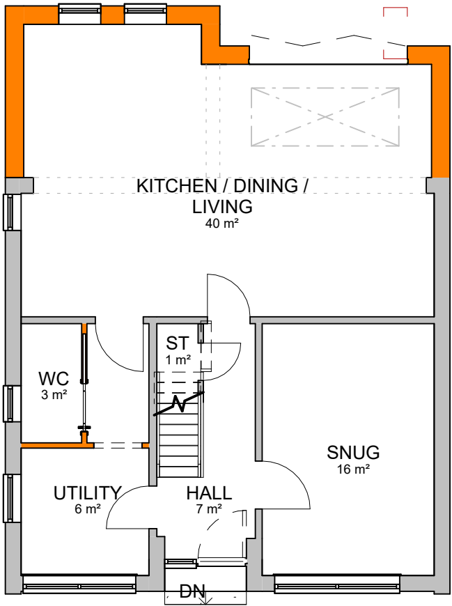
Proposed Ground Floor 1 : 100
