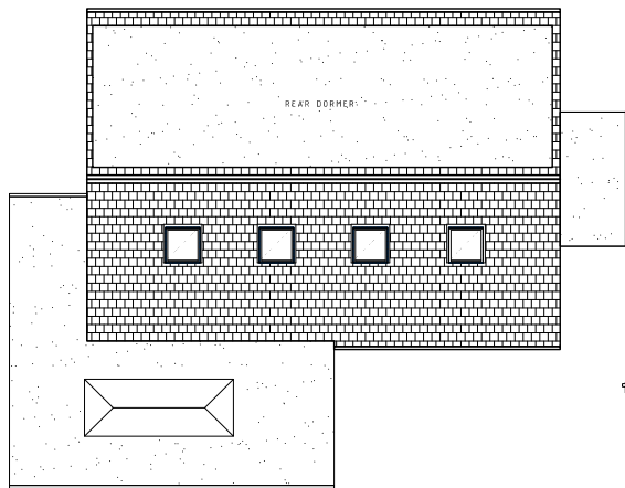
PROPOSED ROOF PLAN 1:200
