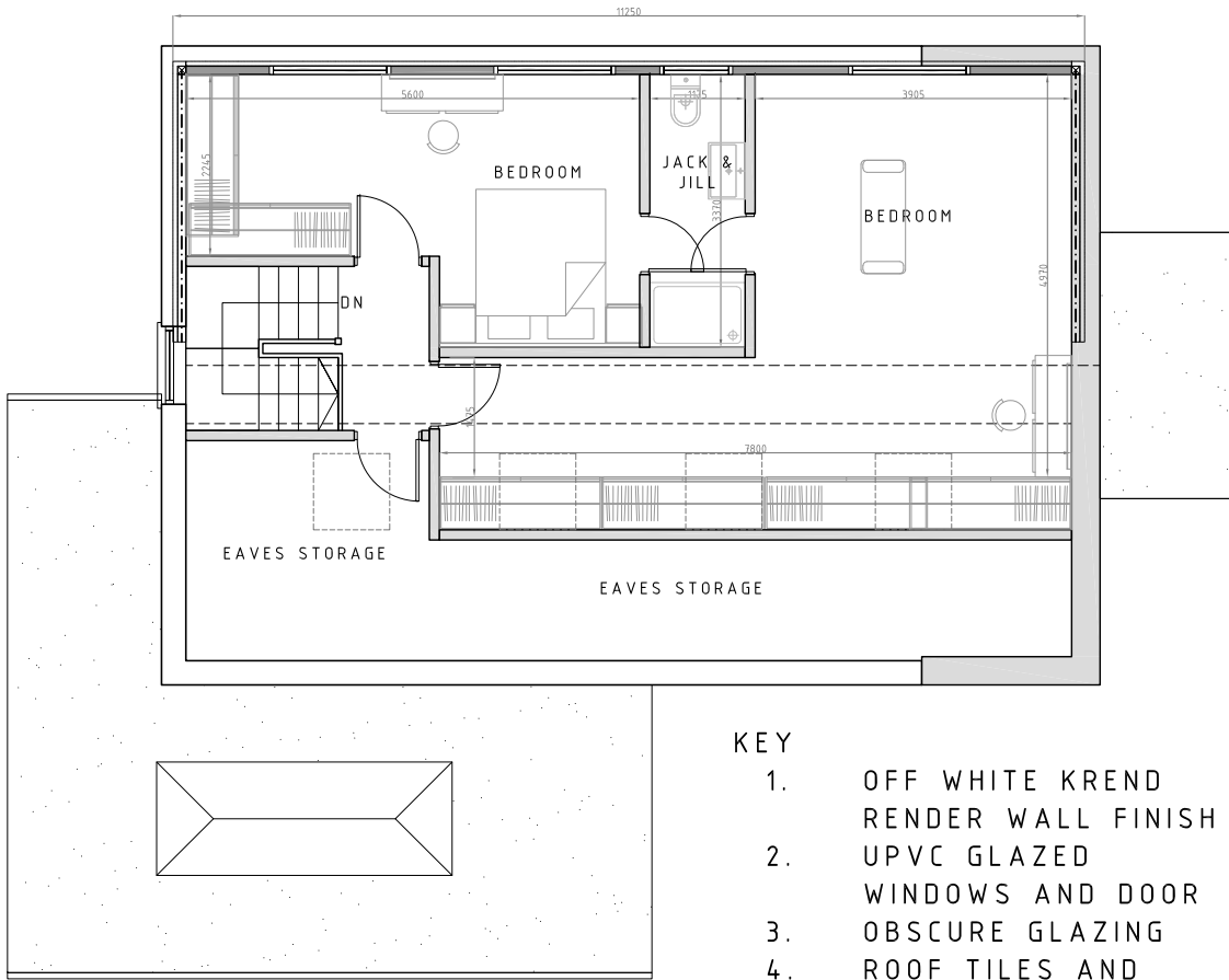
PROPOSED FF PLAN 1:100
