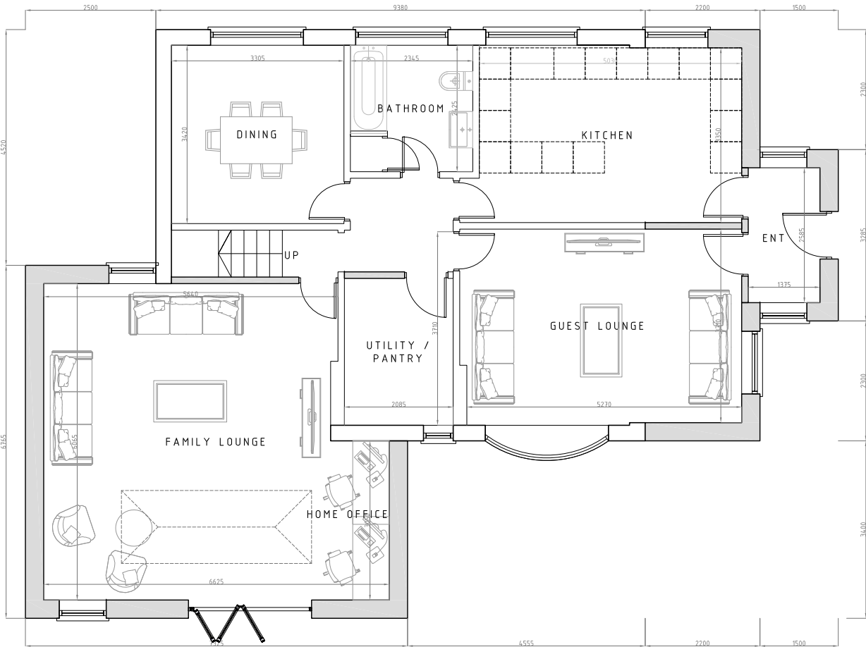
PROPOSED GF PLAN 1:100
