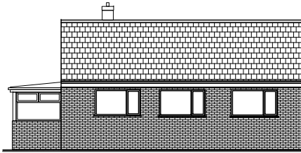
EXISTING REAR ELEV 1:200
