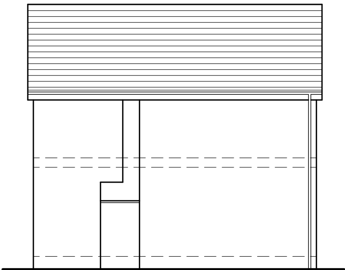
East Elevation
