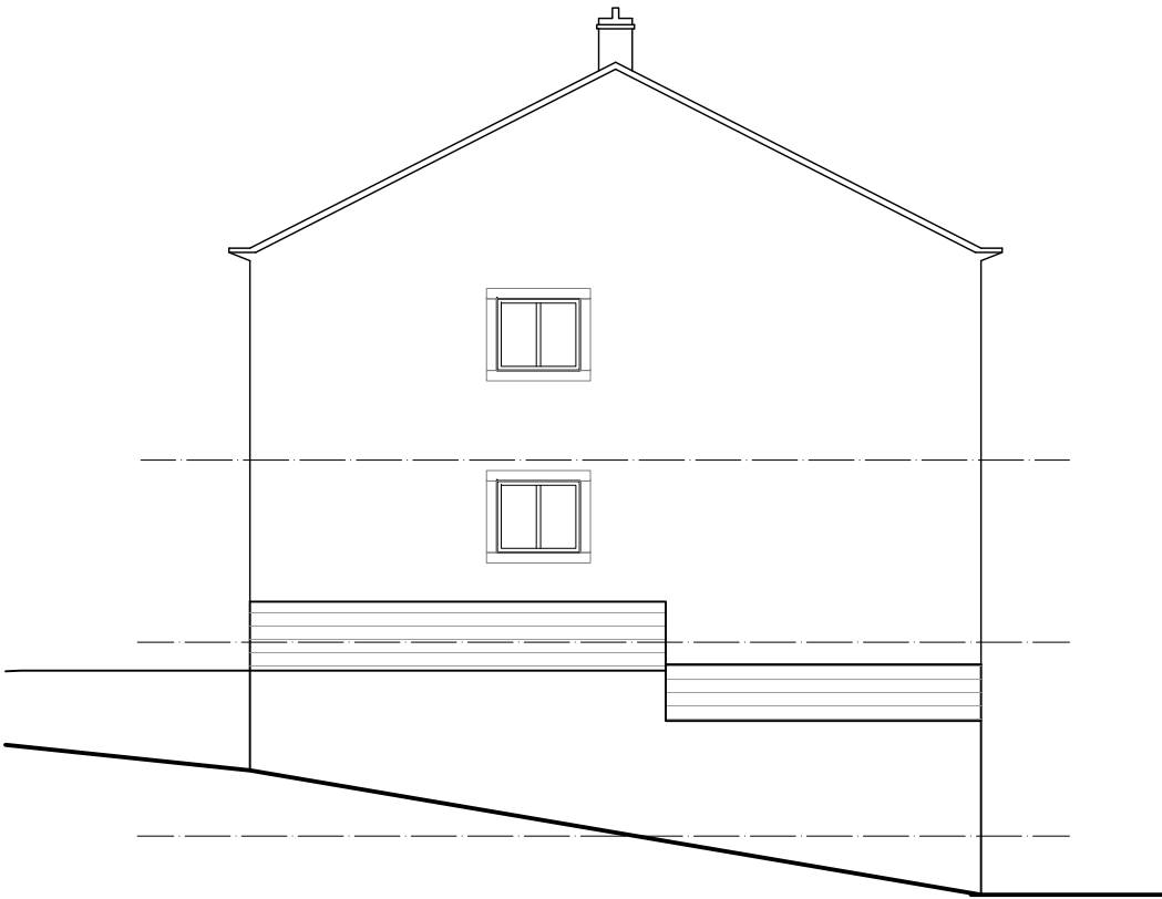
North East (Side) Elevation
