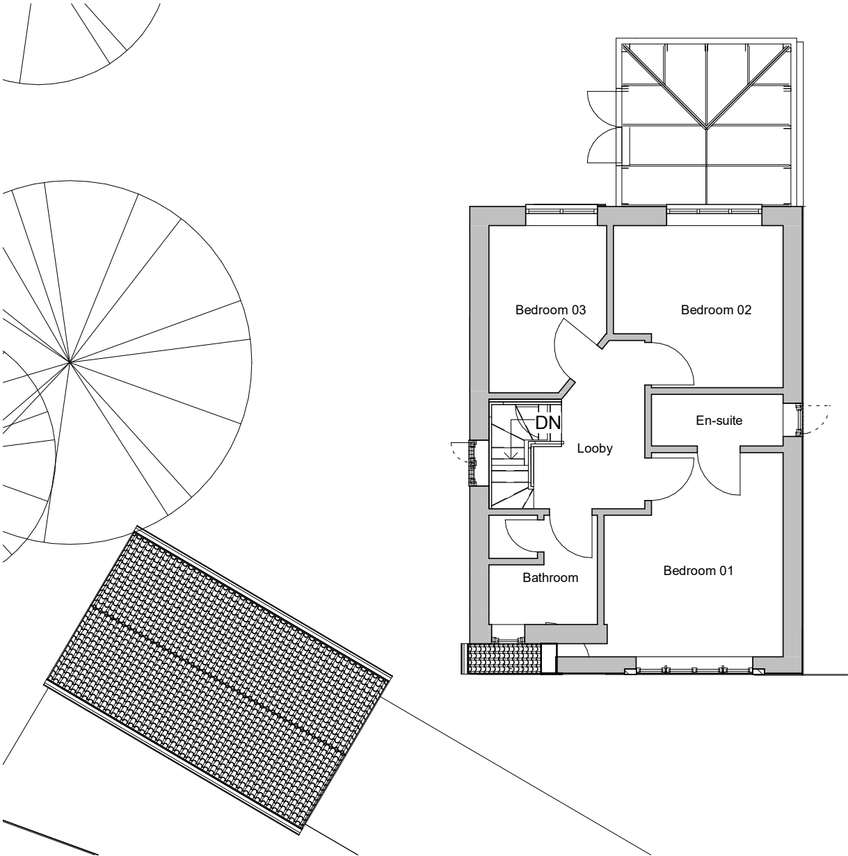
02. First Floor Plan 1 1 : 100
