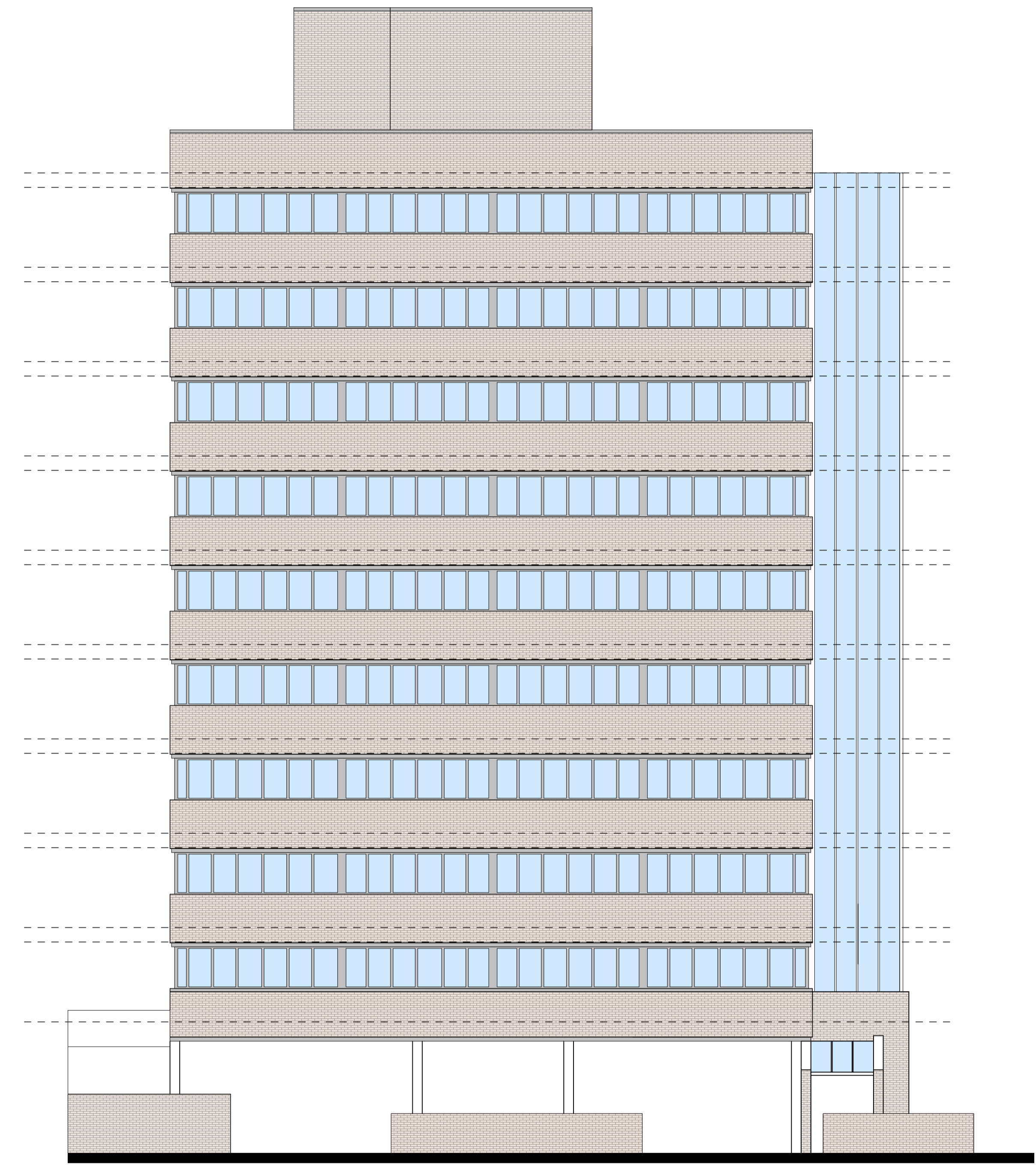
THREADNEEDLE STREET ELEVATION
