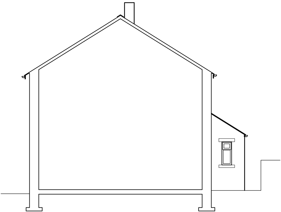
Sectional Elevation (side) East
