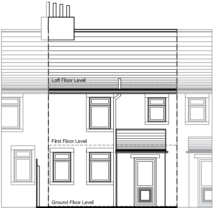
South (front) Elevation
