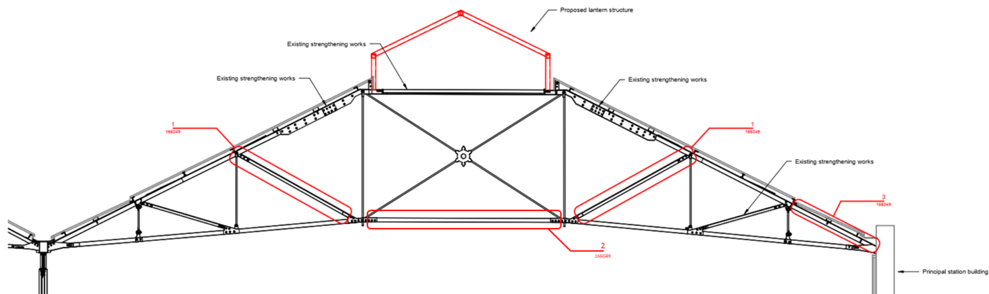
Insert 4-1 Section of retained Roof A, showing the location of the three types of strengthening repairs consented via the granted LBC (full drawings shown in Appendix D).
