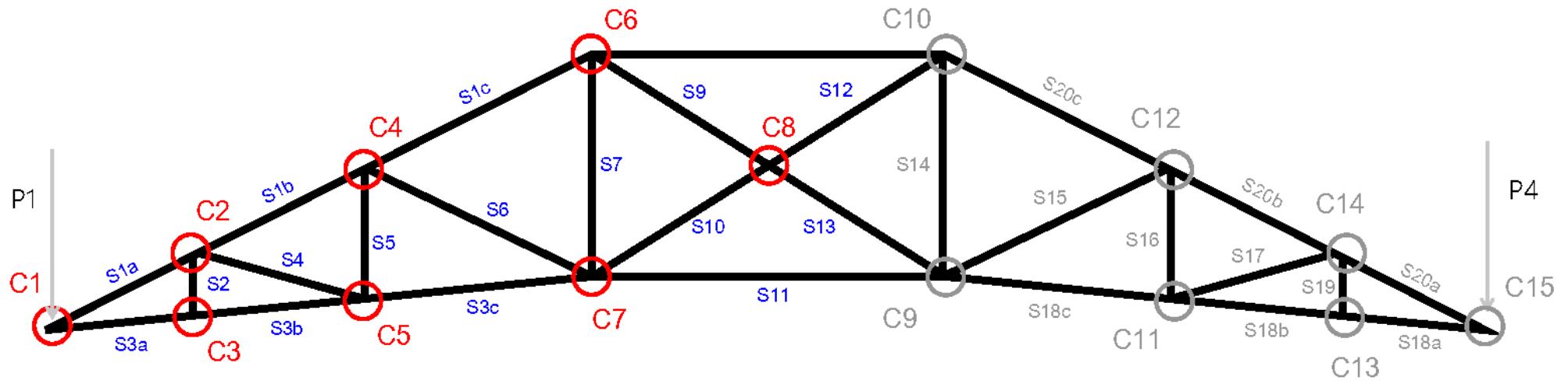
Insert 4-2 Section of retained Roof A, showing the categorisation of truss members and connections for the specification for unforeseen / unexpected repairs. (Note – the station building is to the left)
