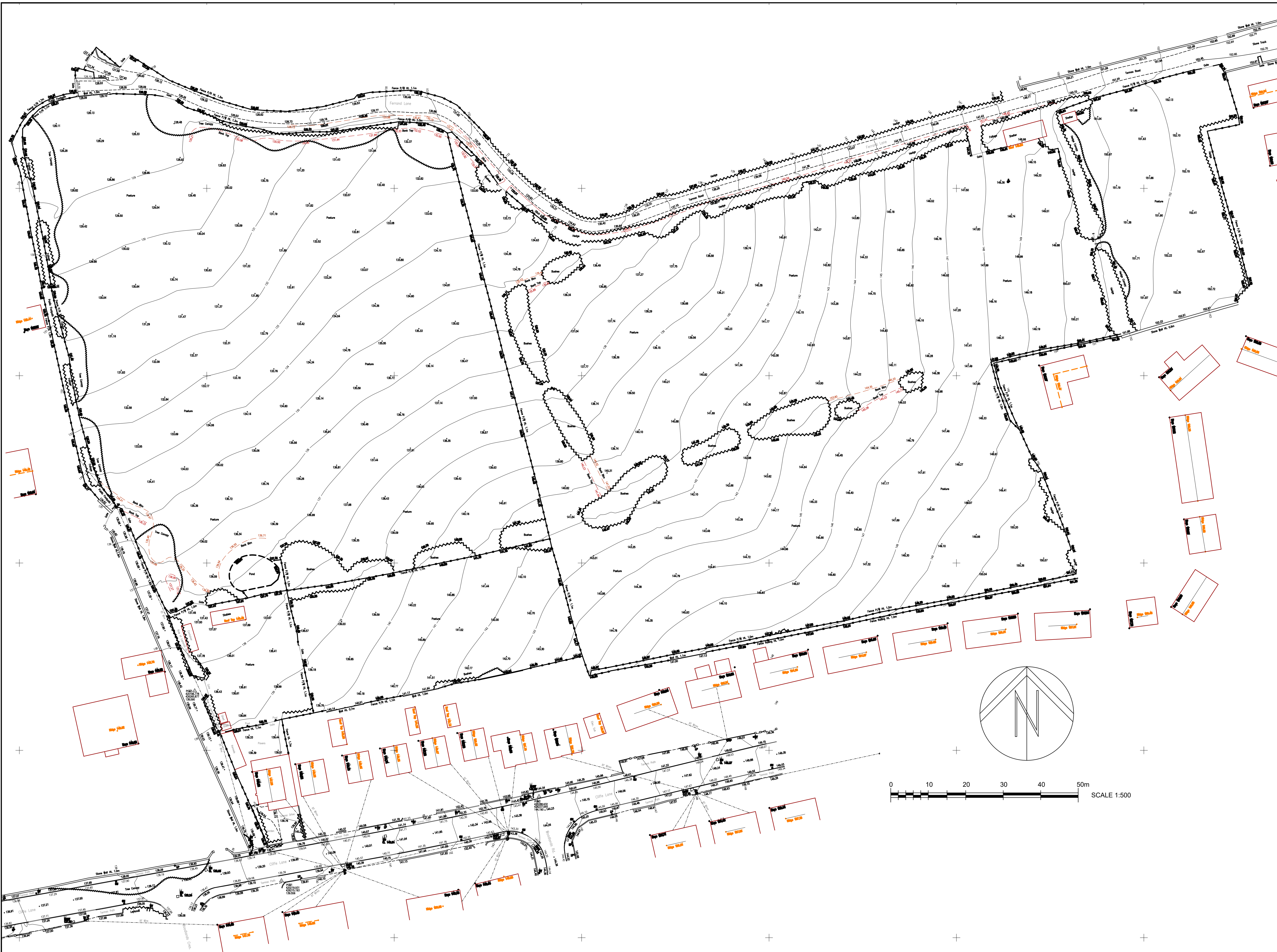
Topographical Survey 1:500
