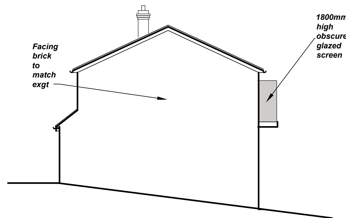
PROPOSED SOUTH EAST ELEVATION Scale 1:100
