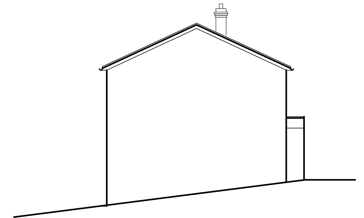
EXISTING NORTH WEST ELEVATION Scale 1:100
