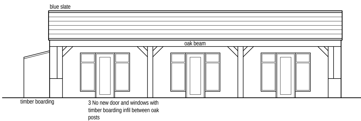
Proposed front/east facing elevation (1:100)
