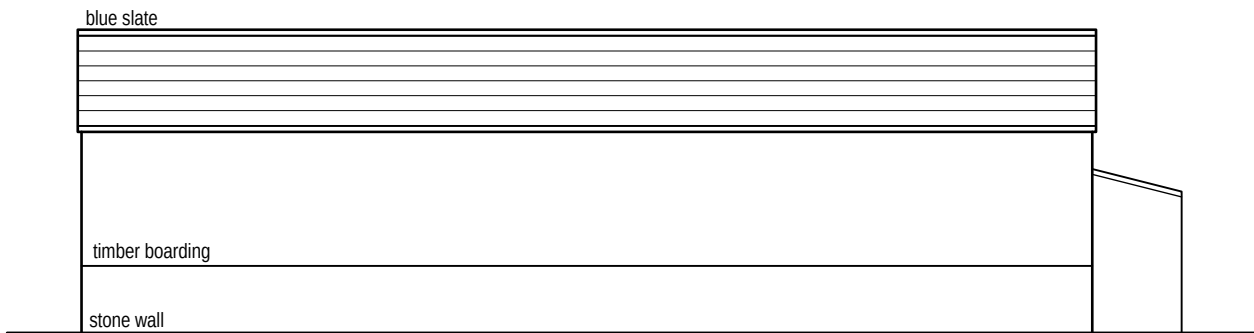
Proposed rear/west facing elevation (1:100)
