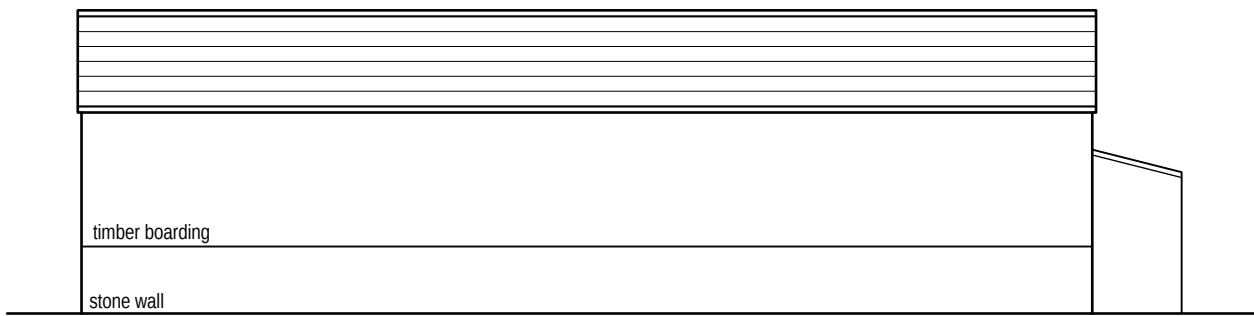
Existing rear/west facing elevation (1:100)
