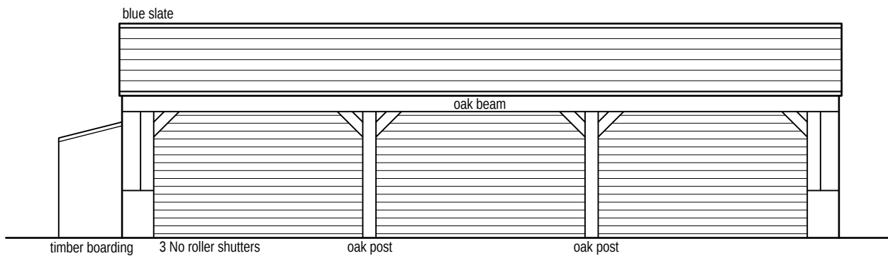
Existing front/east facing elevation (1:100)
