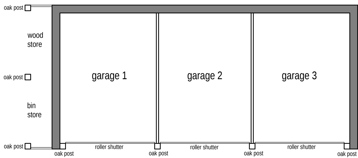
Existing layout (1:100)
