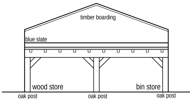
Proposed side/south facing elevation (1:100)
