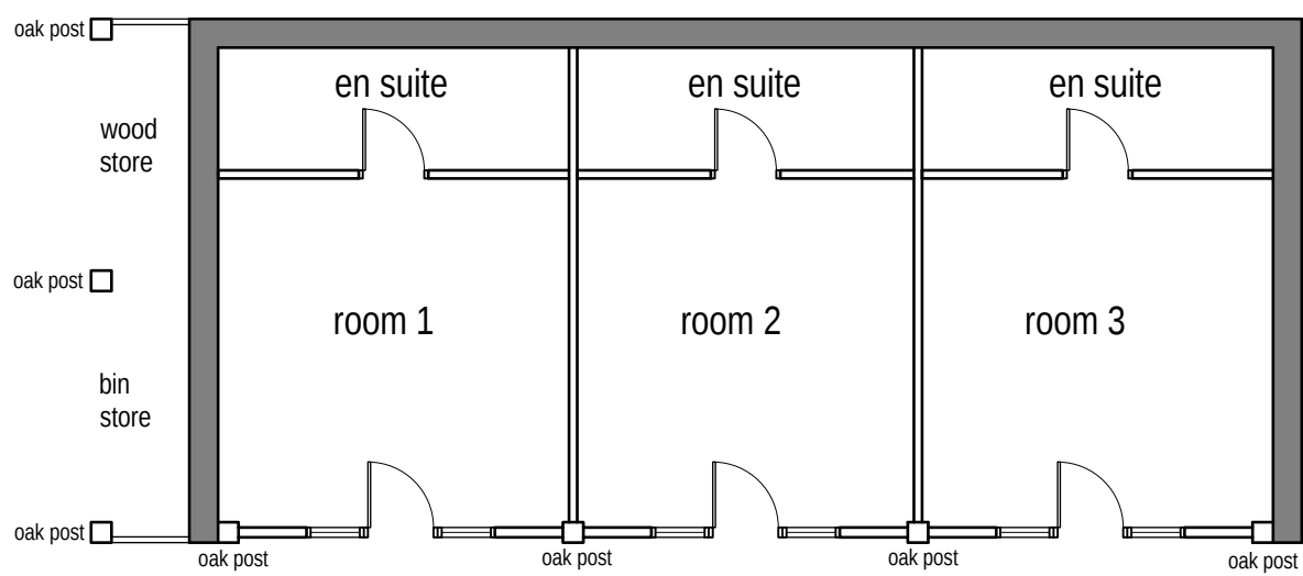
Proposed layout (1:100)
